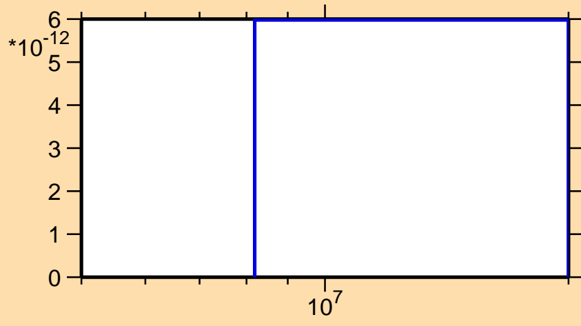
\sigma vs. E for ^{143}\text{Tb} (mt 34)
