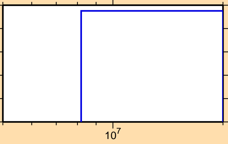
\sigma vs. E for ^{143}\text{Tb}(n,\text{nd})
