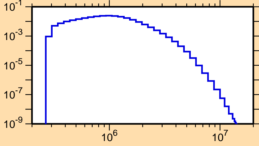
\sigma vs. E for ^{144}\text{Tb}(n,n_2)
