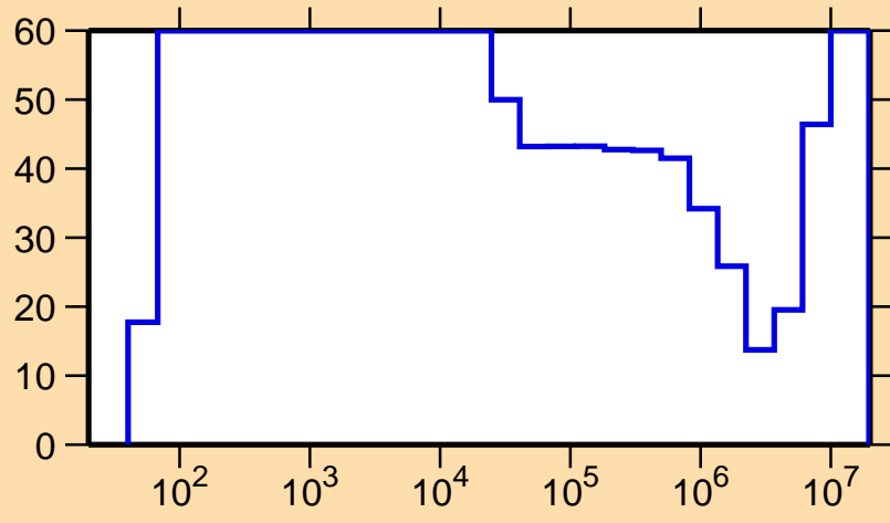
\Delta\sigma/\sigma vs. E for ^{144}\text{Tb}(n,p)
