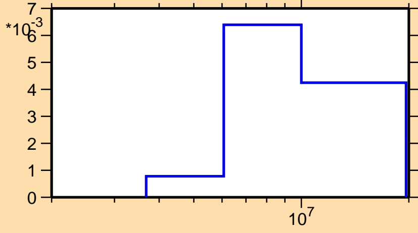
\sigma vs. E for ^{144}\text{Tb}(n,n\text{cont.})
