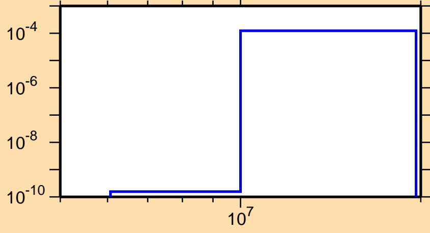
\sigma vs. E for ^{144}\text{Tb} (mt 45)
