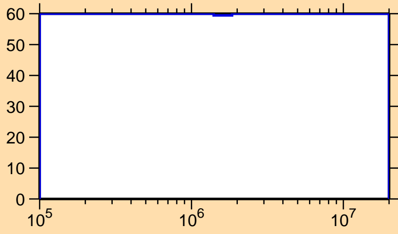
\Delta\sigma/\sigma vs. E for ^{144}\text{Tb}(n,n_1)
