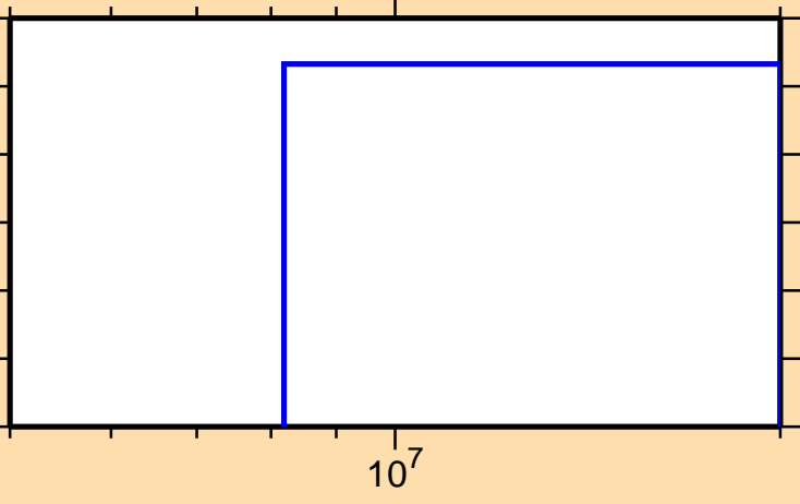
\sigma vs. E for ^{144}\text{Tb}(n,pd)
