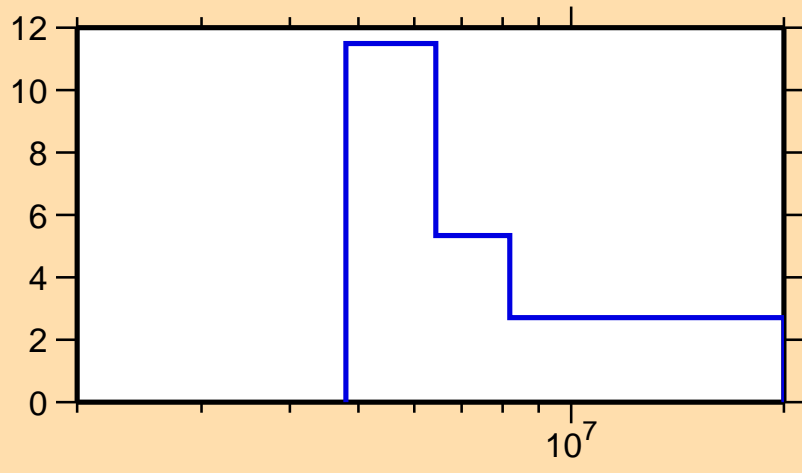
\Delta\sigma/\sigma vs. E for ^{144}\text{Tb}(n,\text{tot.})
