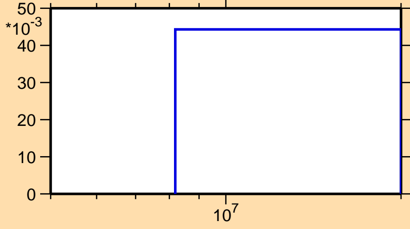
\sigma vs. E for ^{144}\text{Tb}(n,2n)
