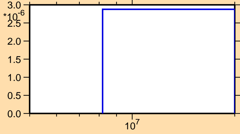
\sigma vs. E for ^{144}\text{Tb}(n,\text{nd})
