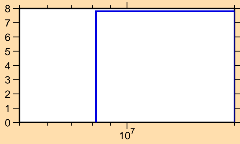
\Delta\sigma/\sigma vs. E for ^{144}\text{Tb}(n,\text{el.})
