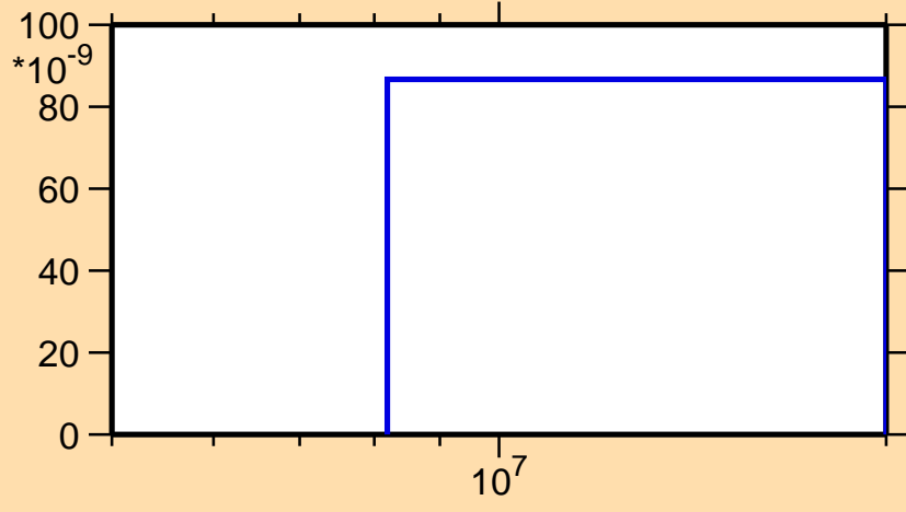
\sigma vs. E for ^{144}\text{Tb}(n,\text{pt})
