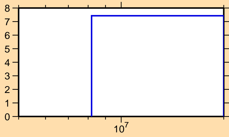
\Delta\sigma/\sigma vs. E for ^{144}\text{Tb}(n,\text{nonel.})
