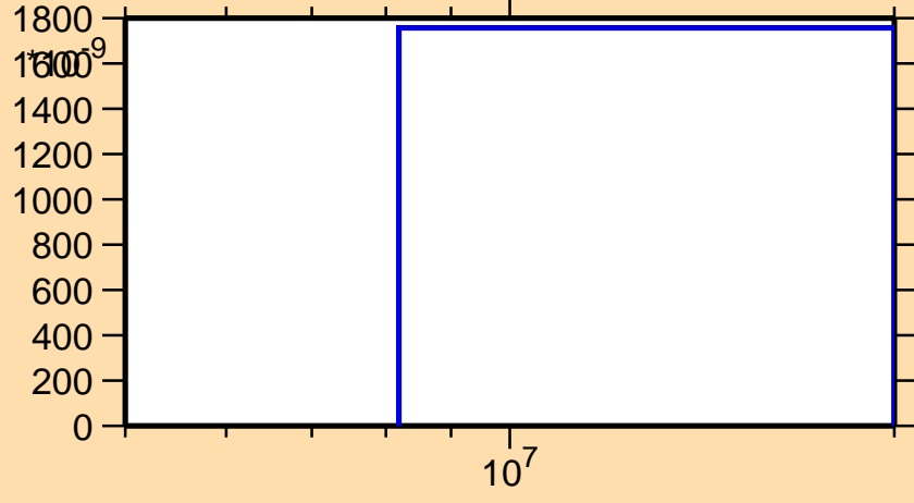
\sigma vs. E for ^{144}\text{Tb}(n,2n\alpha)
