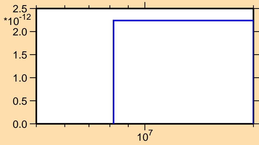
\sigma vs. E for ^{144}\text{Tb}(n,nt)
