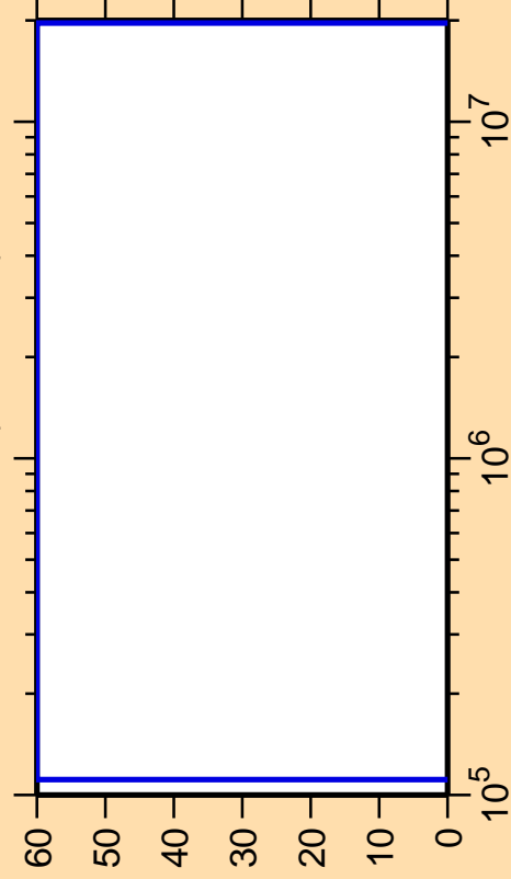
\Delta\sigma/\sigma vs. E for ^{144}\text{Tb}(n,n\text{cont.})
