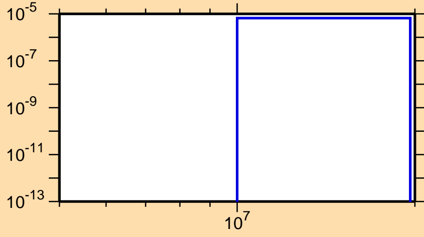
\sigma vs. E for ^{144}\text{Tb}(n,p,d)
