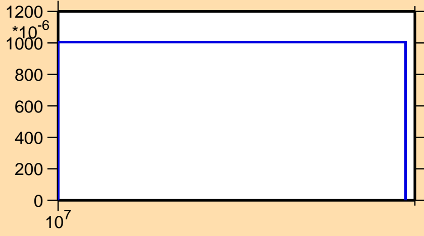
\sigma vs. E for ^{144}\text{Tb}(n,2np)
