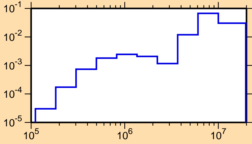
\sigma vs. E for ^{144}\text{Tb}(n,n\text{cont.})
