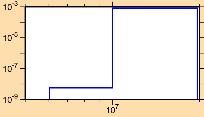
\sigma vs. E for ^{144}\text{Tb}(n,t)
