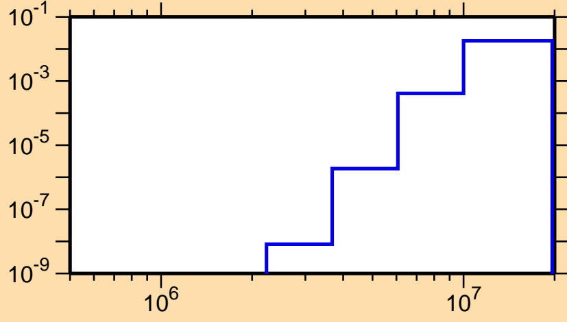
\sigma vs. E for ^{144}\text{Tb}(n,d)
