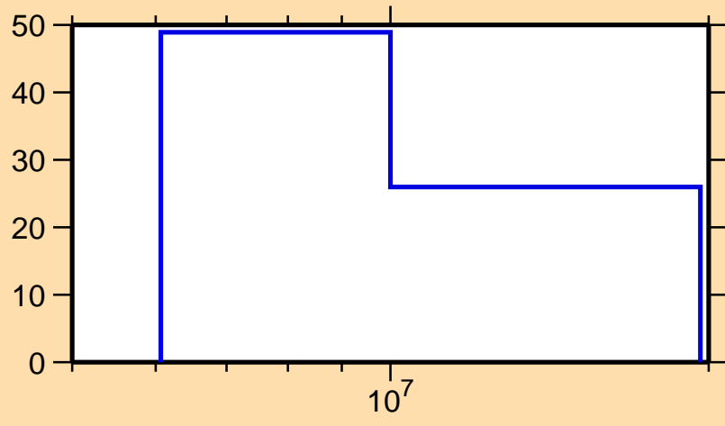
\Delta\sigma/\sigma vs. E for ^{144}\text{Tb}(n,\text{el.})
