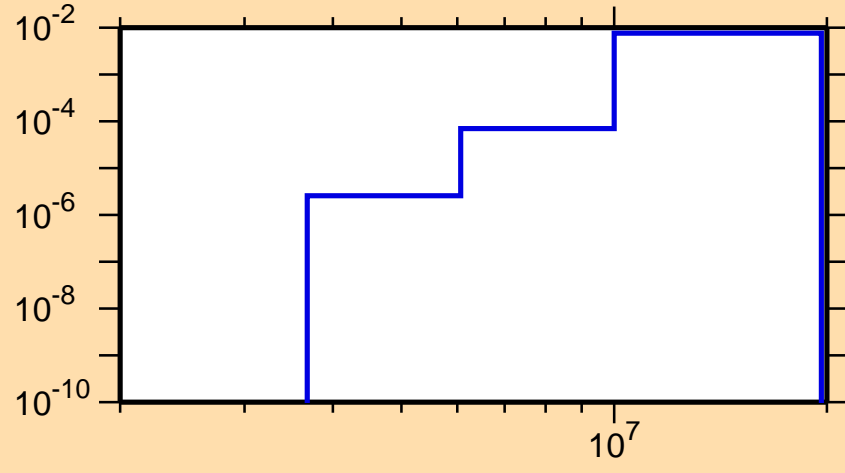
\sigma vs. E for ^{144}\text{Tb}(n,n\alpha)
