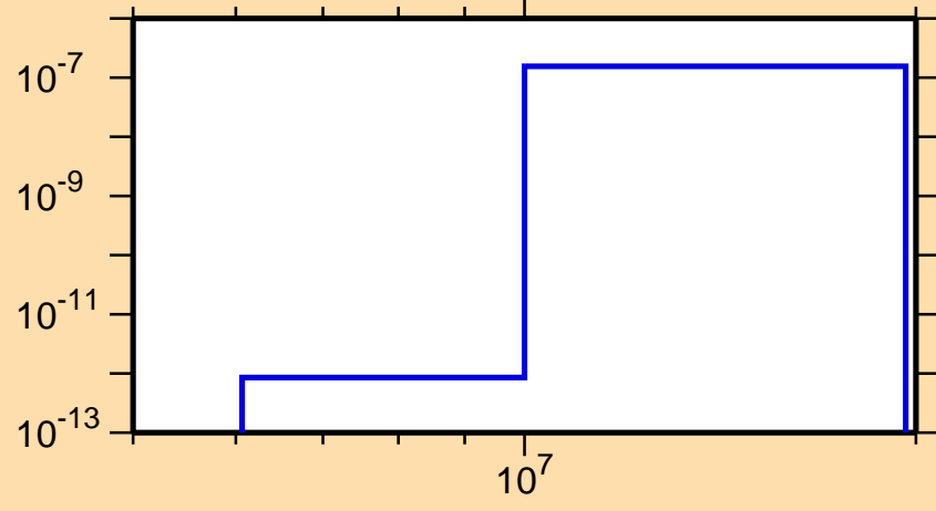
\sigma vs. E for ^{144}\text{Tb}(\text{mt117})
