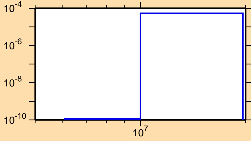
\sigma vs. E for ^{144}\text{Tb} (mt 45)
