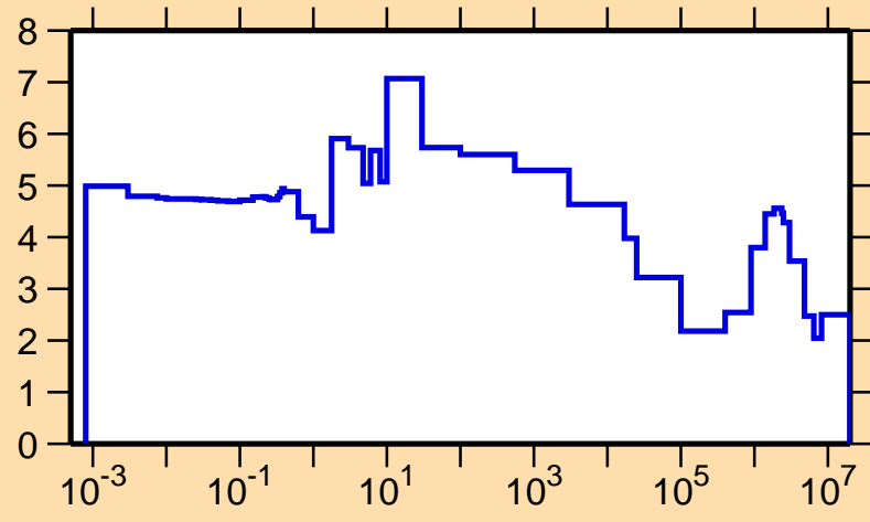
\sigma vs. E for ^{144}\text{Tb}(n,\text{el.})
