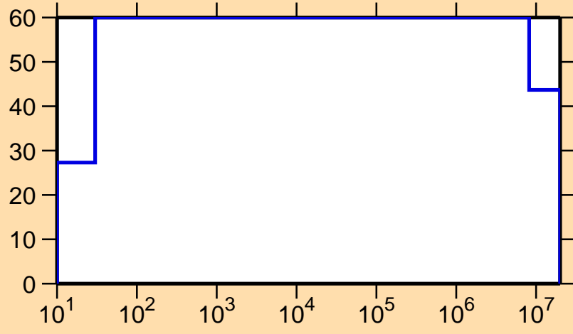
\Delta\sigma/\sigma vs. E for ^{144}\text{Tb}(n,\gamma)
