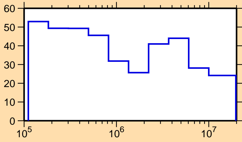
\Delta\sigma/\sigma vs. E for ^{145}\text{Tb}(n,n_1)
