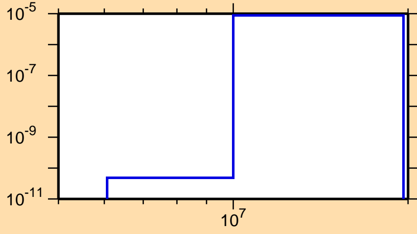
\sigma vs. E for ^{145}\text{Tb}(n,\text{He3})
