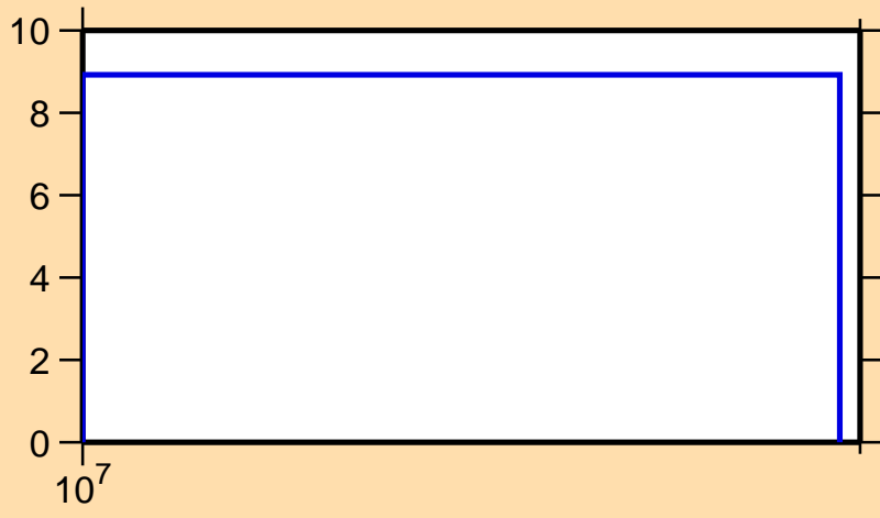
\Delta\sigma/\sigma vs. E for ^{145}\text{Tb}(n,\text{el.})
