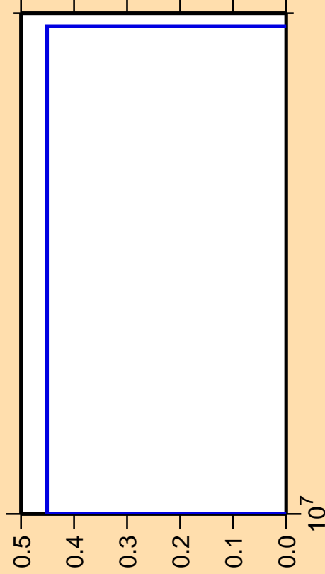
\Delta\sigma/\sigma vs. E for ^{145}\text{Tb} (mt 34)
