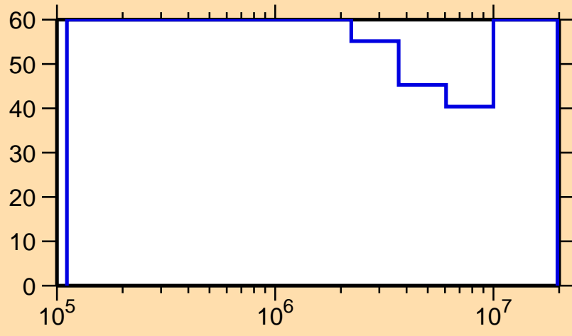
\Delta\sigma/\sigma vs. E for ^{145}\text{Tb}(n,n\text{cont.})
