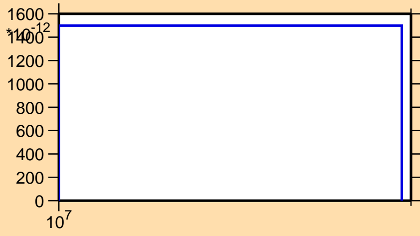
\sigma vs. E for ^{145}\text{Tb}(n,2n\alpha)
