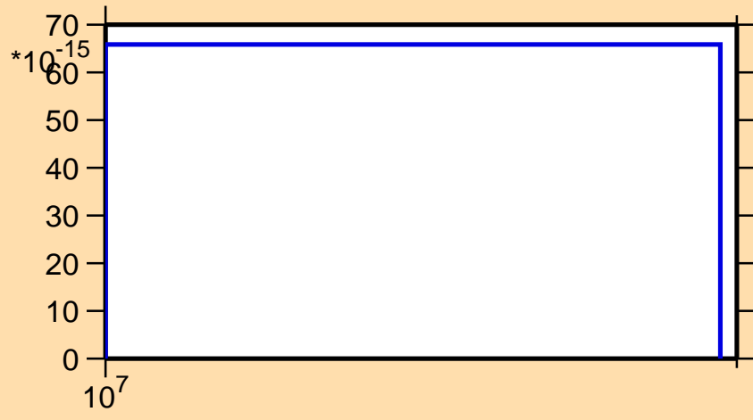
\sigma vs. E for ^{145}\text{Tb} (mt 34)
