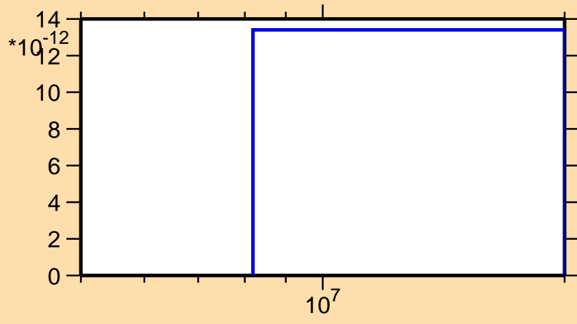
\sigma vs. E for ^{145}\text{Tb}(n,\text{pt})
