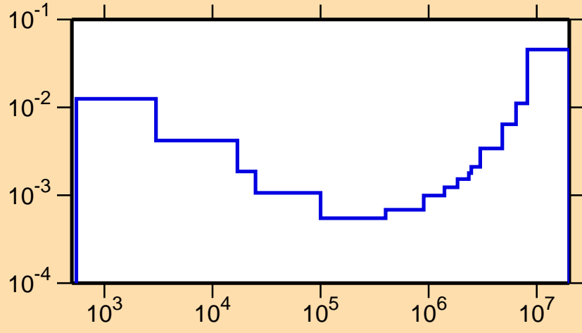
\sigma vs. E for ^{145}\text{Tb}(n,\alpha)
