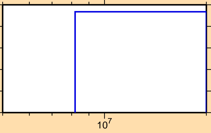
\sigma vs. E for ^{145}\text{Tb}(n,\text{pd})
