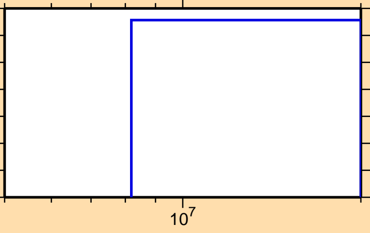
\sigma vs. E for ^{145}\text{Tb}(n,2np)
