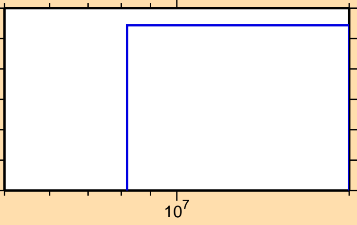
\sigma vs. E for ^{145}\text{Tb}(n,\text{nd})
