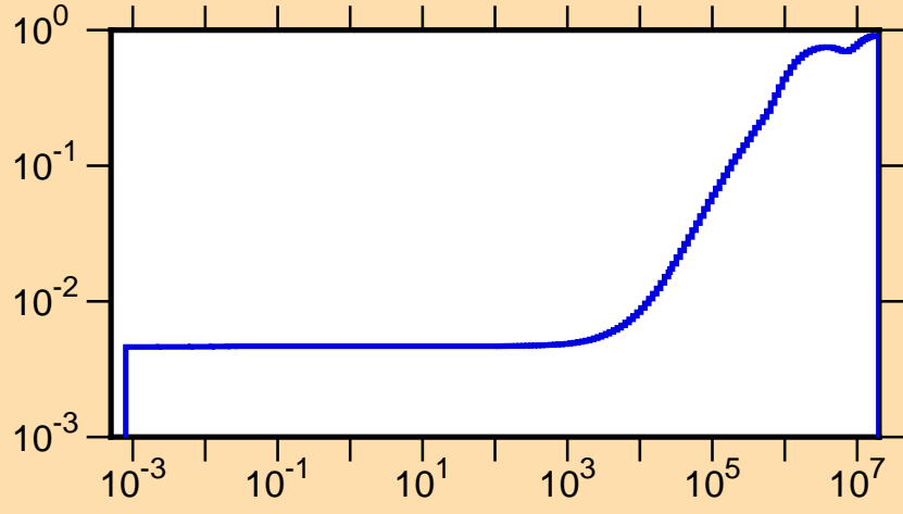
\mu vs. E for ^{146}\text{Tb}(\text{mt251})
