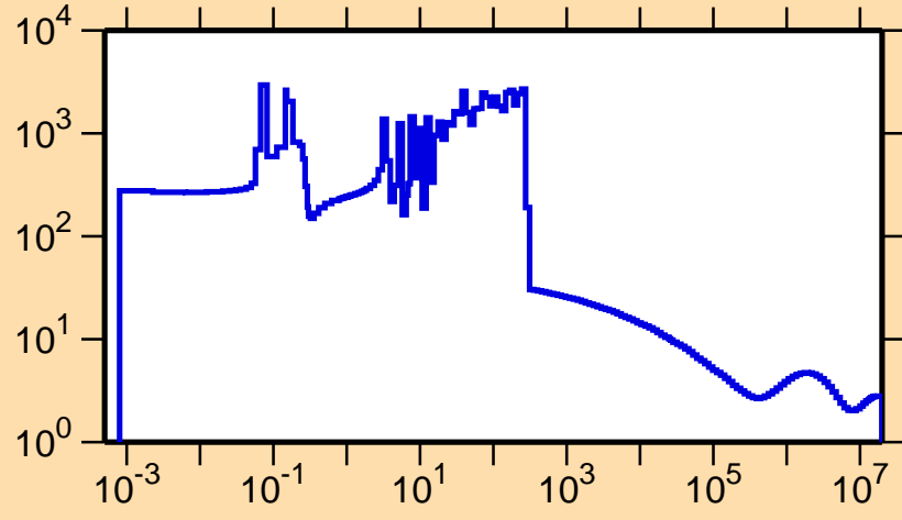
\sigma vs. E for ^{146}\text{Tb}(n,\text{el.})
