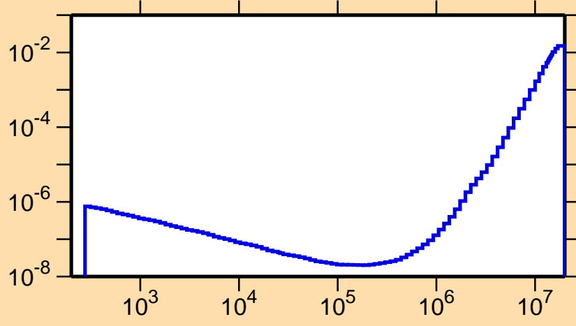
\sigma vs. E for ^{146}\text{Tb}(n,p\alpha)
