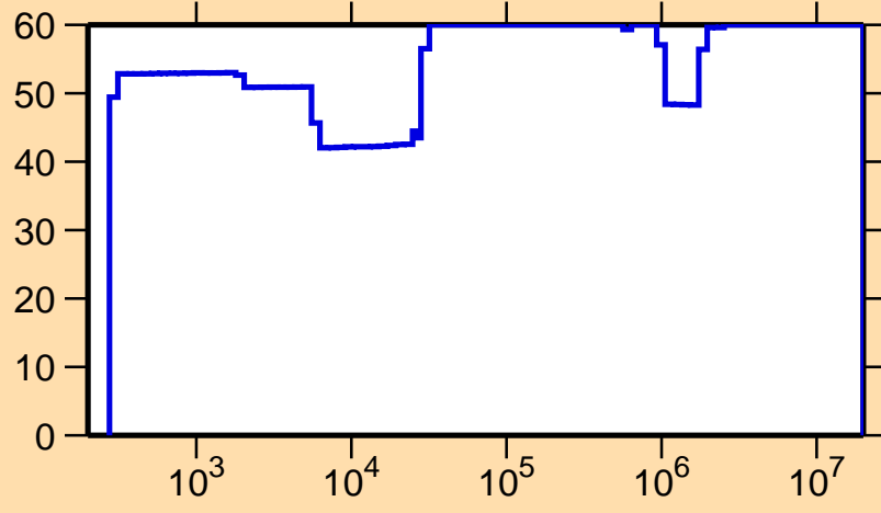
\Delta\sigma/\sigma vs. E for ^{146}\text{Tb}(n,p)
