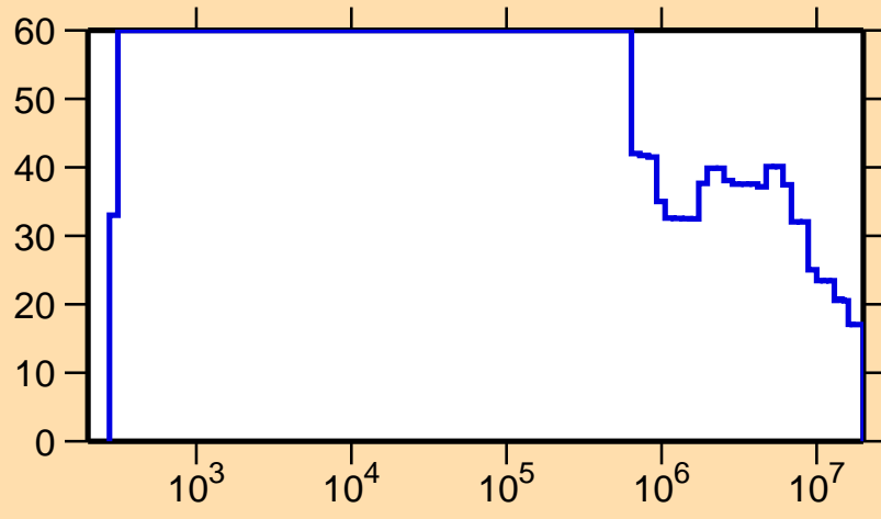
\Delta\sigma/\sigma vs. E for ^{146}\text{Tb}(n,el.)
