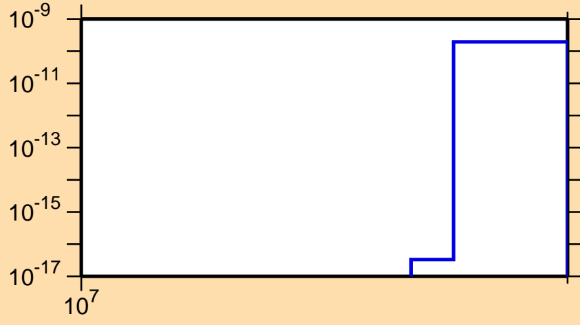
\sigma vs. E for ^{146}\text{Tb}(n,nt)
