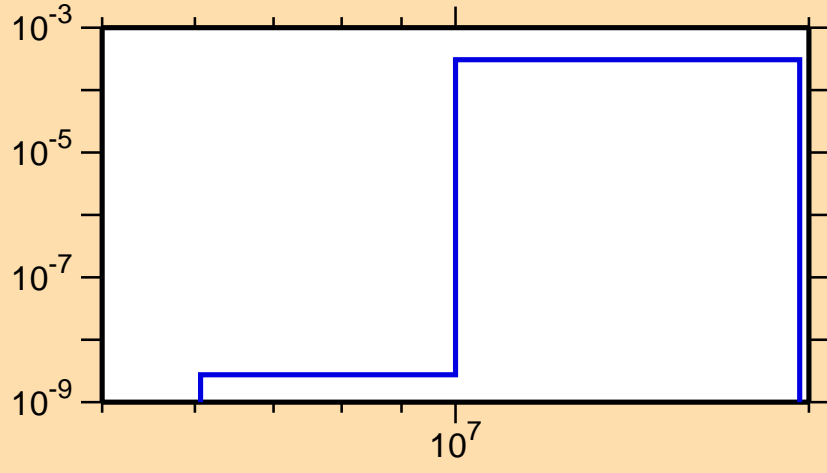
\sigma vs. E for ^{146}\text{Tb}(n,t)
