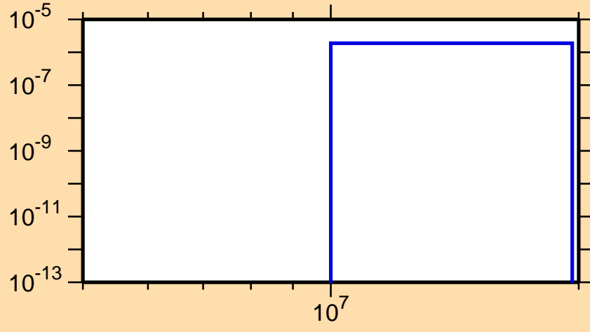
\sigma vs. E for ^{146}\text{Tb} (mt 45)
