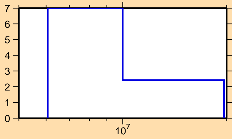
\Delta\sigma/\sigma vs. E for ^{146}\text{Tb}(n,\text{nonel.})
