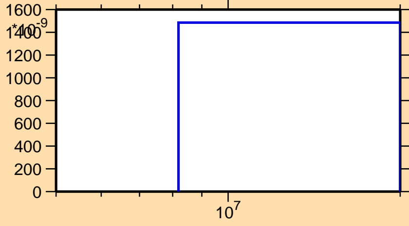
\sigma vs. E for ^{146}\text{Tb}(n,\text{pd})
