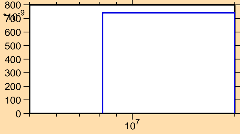
\sigma vs. E for ^{146}\text{Tb}(n,pd)
