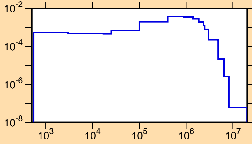
\sigma vs. E for ^{146}\text{Tb}(n,n_1)
