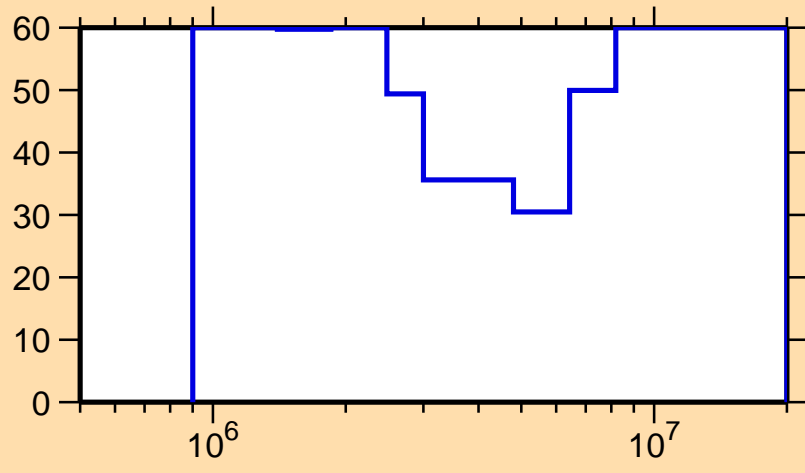
\Delta\sigma/\sigma vs. E for ^{146}\text{Tb}(n,n\text{cont.})
