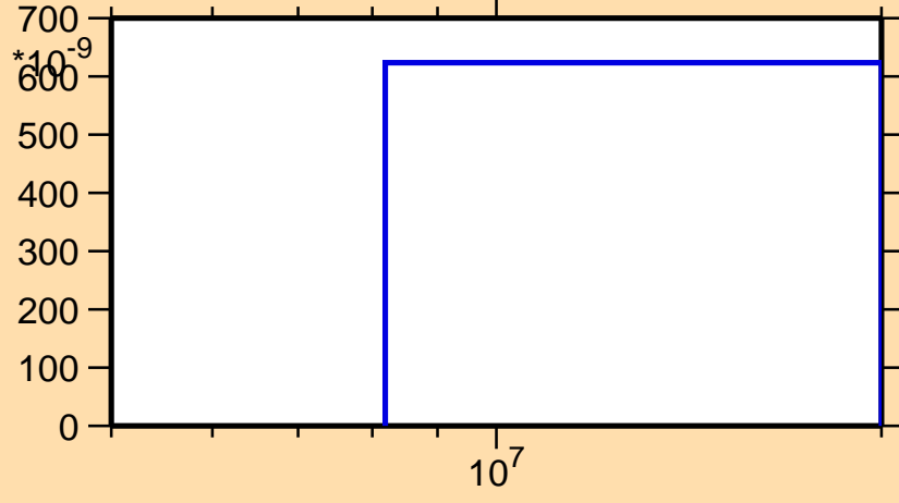
\sigma vs. E for ^{146}\text{Tb}(n,\text{nd})
