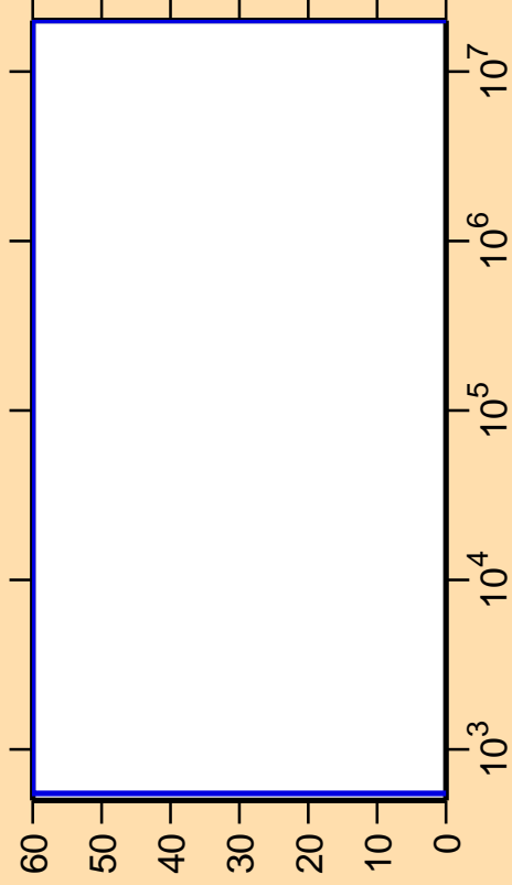
\Delta\sigma/\sigma vs. E for ^{146}\text{Tb}(n,p\alpha)
