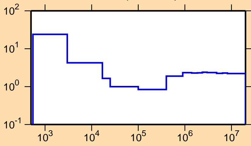
\sigma vs. E for ^{147}\text{Tb}(n,\text{nonel.})
