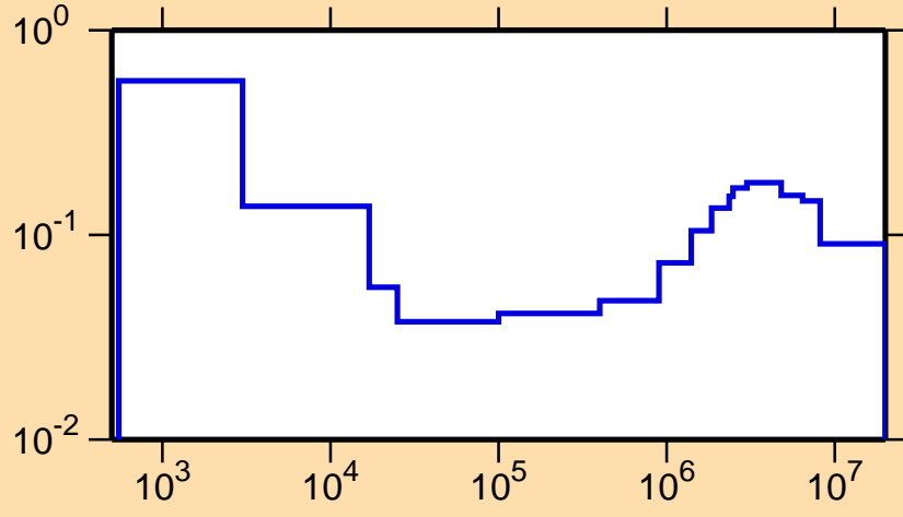
\sigma vs. E for ^{147}\text{Tb}(n,p)
