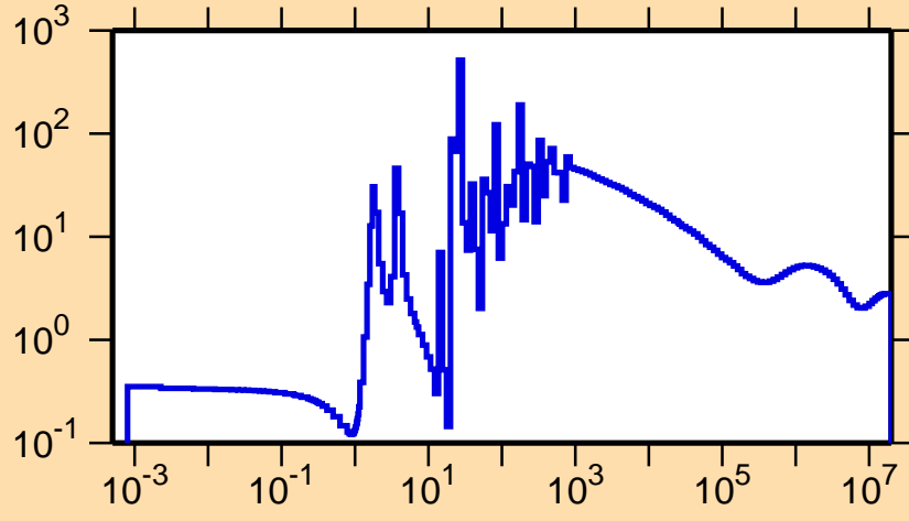
\sigma vs. E for ^{147}\text{Tb}(n,\text{el.})
