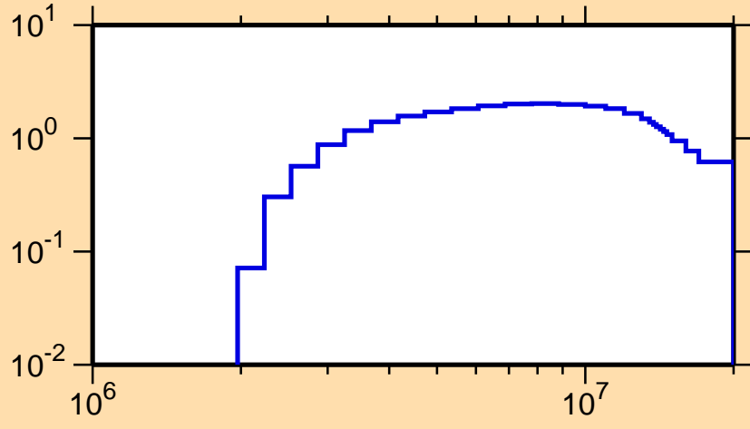
\sigma vs. E for ^{147}\text{Tb}(n,n\text{cont.})
