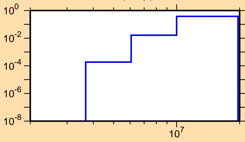
\sigma vs. E for ^{147}\text{Tb}(n,np)
