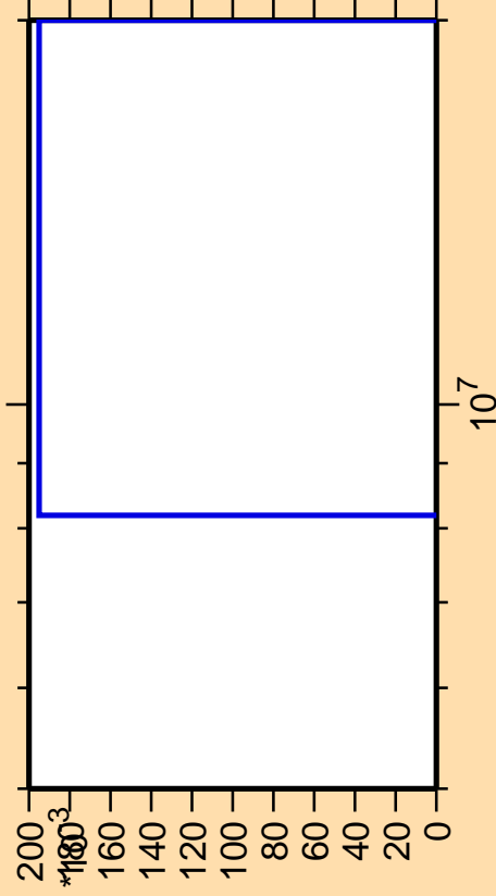
\Delta\sigma/\sigma vs. E for ^{147}\text{Tb} (mt 34)
