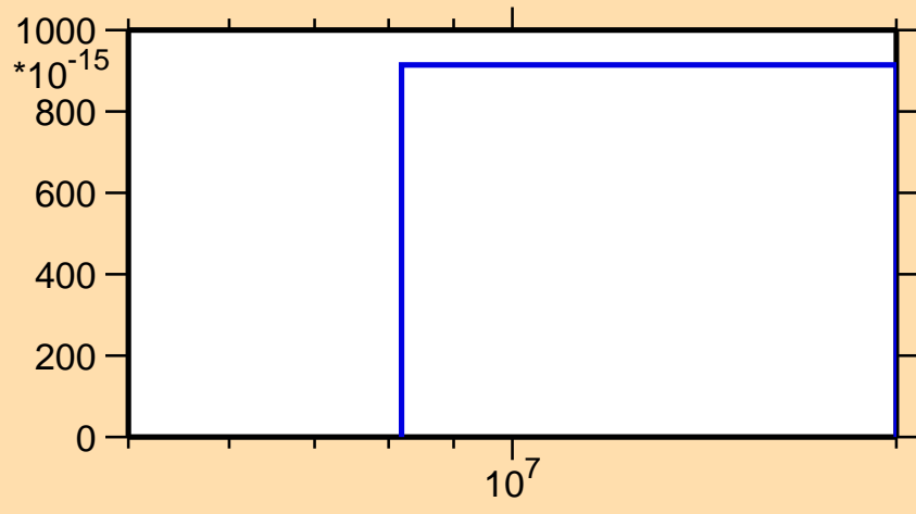
\sigma vs. E for ^{147}\text{Tb}(n,nt)
