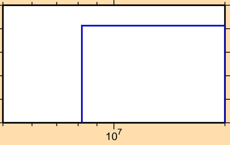
\sigma vs. E for ^{148}\text{Tb}(n,nt)
