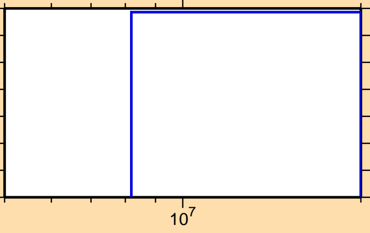
\sigma vs. E for ^{148}\text{Tb}(n,pd)
