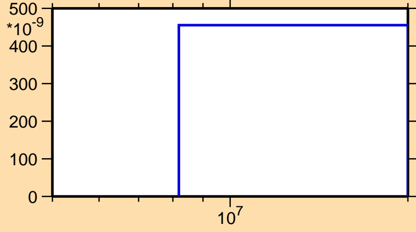
\sigma vs. E for ^{148}\text{Tb} (mt 45)
