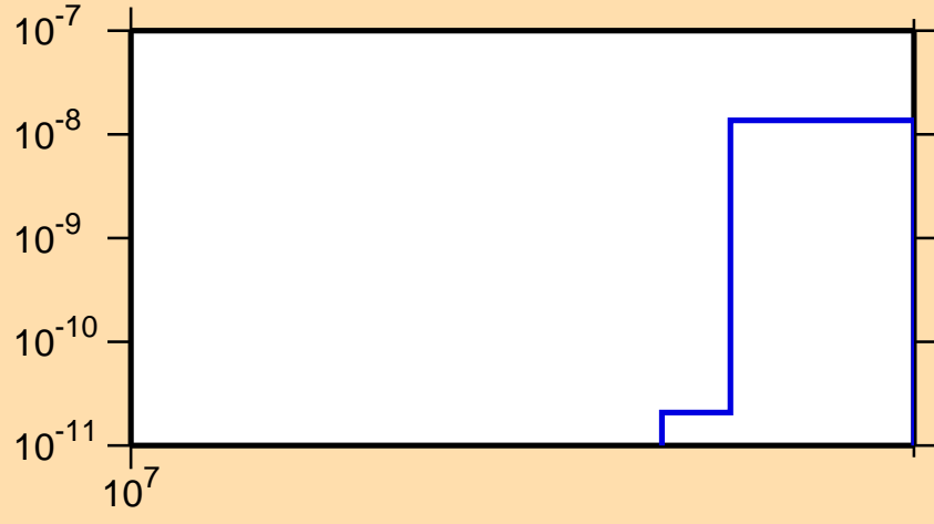
\sigma vs. E for ^{148}\text{Tb}(n,nt)
