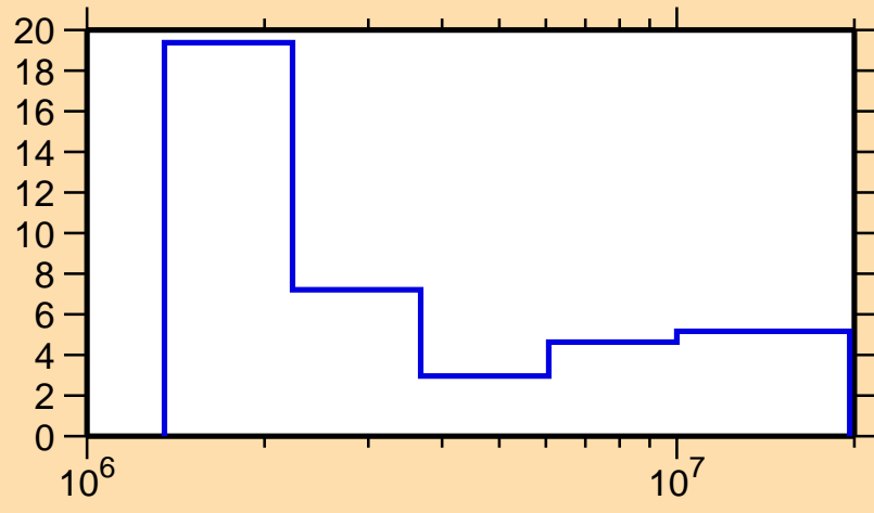
\Delta\sigma/\sigma vs. E for ^{148}\text{Tb}(n,n\text{onel.})
