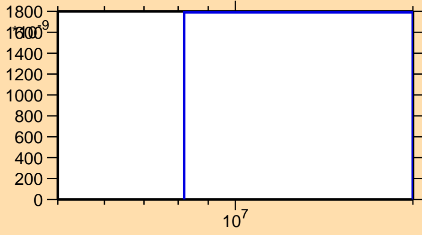
\sigma vs. E for ^{148}\text{Tb}(n,\text{nd})
