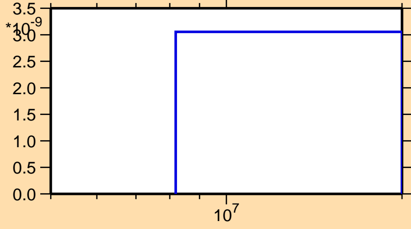
\sigma vs. E for ^{148}\text{Tb}(n,pd)
