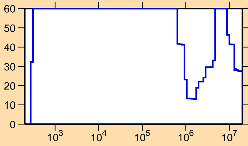
\Delta\sigma/\sigma vs. E for ^{149}\text{Tb}(n,el.)
