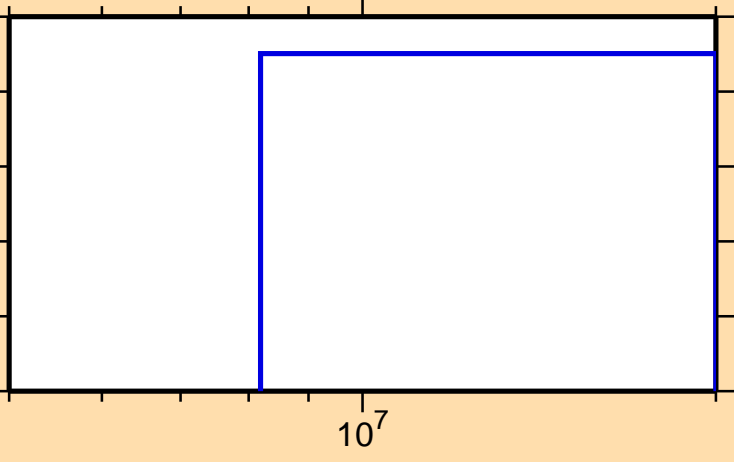
\sigma vs. E for ^{149}\text{Tb}(n,2n\alpha)
