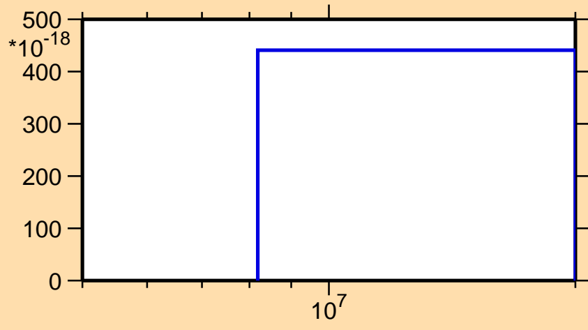
\sigma vs. E for ^{149}\text{Tb}(\text{mt } 11)
