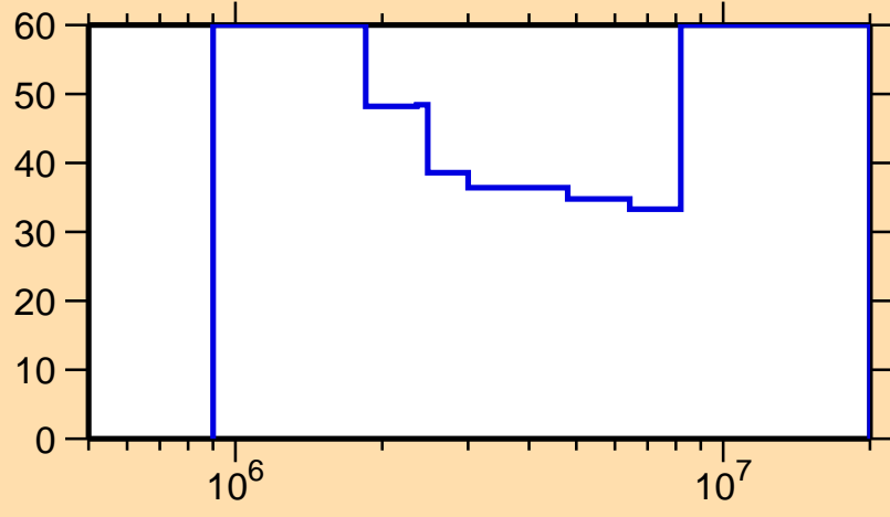
\Delta\sigma/\sigma vs. E for ^{149}\text{Tb}(n,n\text{cont.})
