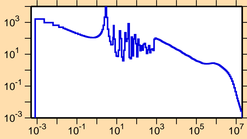
\sigma vs. E for ^{149}\text{Tb}(n,\gamma)
