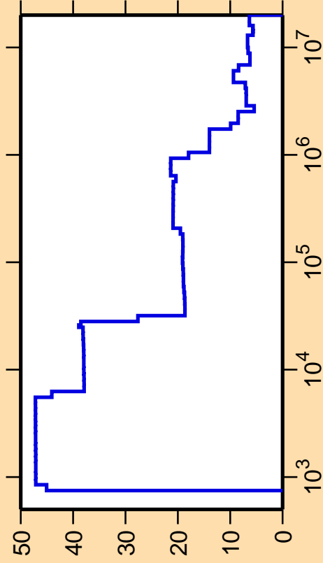
\Delta\sigma/\sigma vs. E for ^{149}\text{Tb}(n,\text{nonel.})
