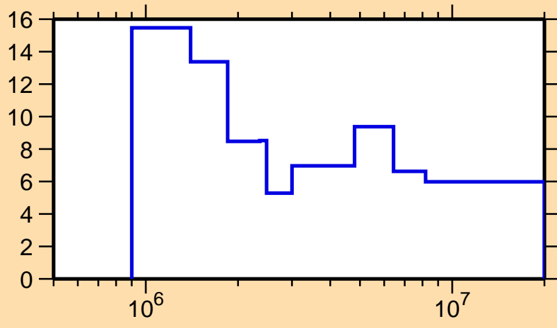
\Delta\sigma/\sigma vs. E for ^{149}\text{Tb}(n,n\text{onel.})
