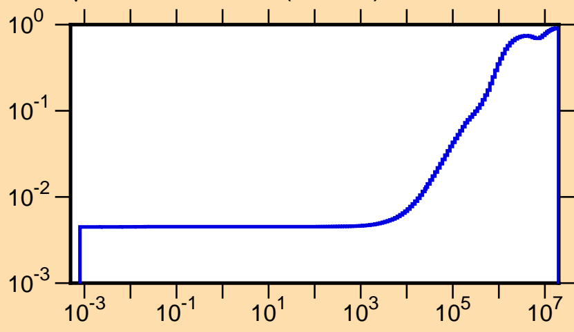
\mu vs. E for ^{150}\text{Tb}(\text{mt251})
