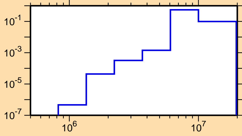
\sigma vs. E for ^{150}\text{Tb}(n,n\text{cont.})
