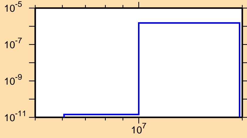
\sigma vs. E for ^{150}\text{Tb}(\text{mt } 45)
