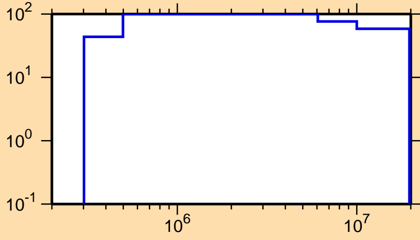
\Delta\sigma/\sigma vs. E for ^{150}\text{Tb}(n,n\text{cont.})
