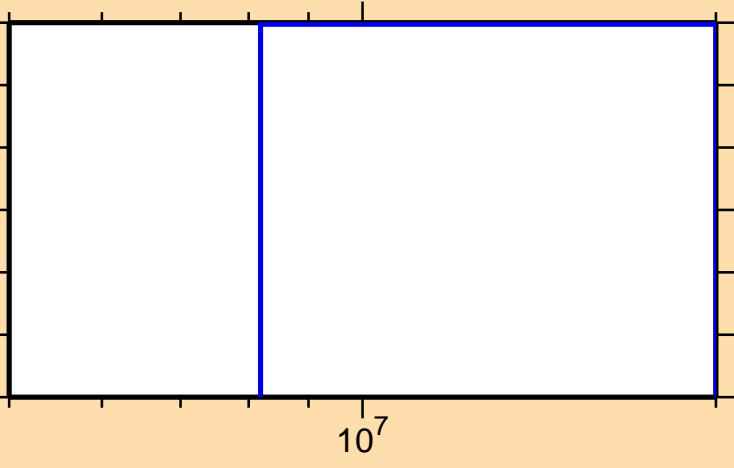
\sigma vs. E for ^{150}\text{Tb} (mt 34)
