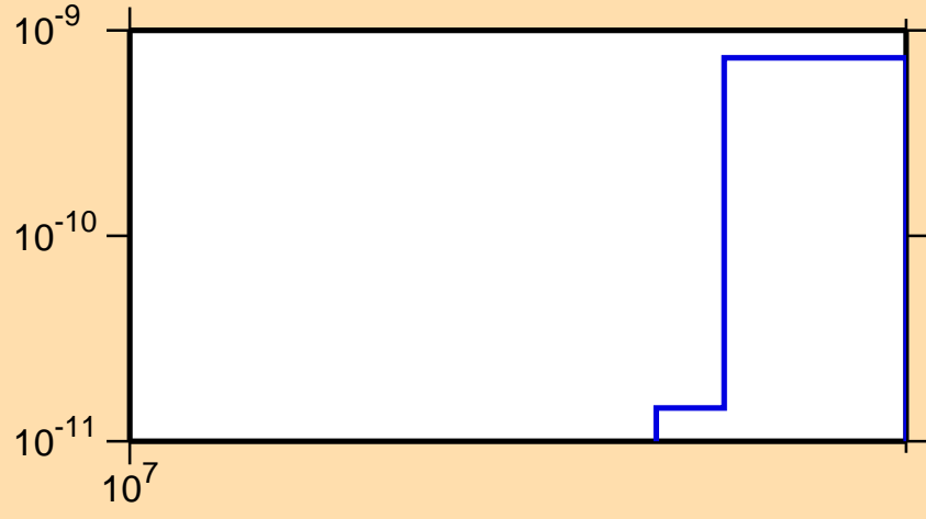
\sigma vs. E for ^{150}\text{Tb} (mt 34)
