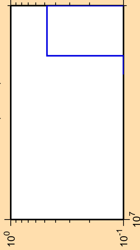
\Delta\sigma/\sigma vs. E for ^{150}\text{Tb}(n,3n\alpha)
