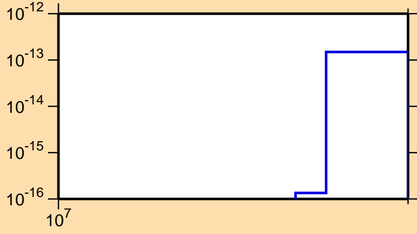
\sigma vs. E for ^{150}\text{Tb} (mt 11)
