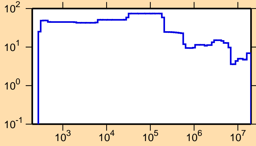
\Delta\sigma/\sigma vs. E for ^{150}\text{Tb}(n,el.)
