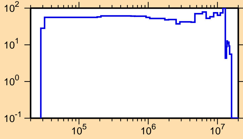
\Delta\sigma/\sigma vs. E for ^{150}\text{Tb}(n,n_1)
