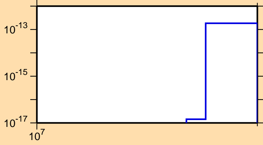
\sigma vs. E for ^{150}\text{Tb}(n,3n\alpha)
