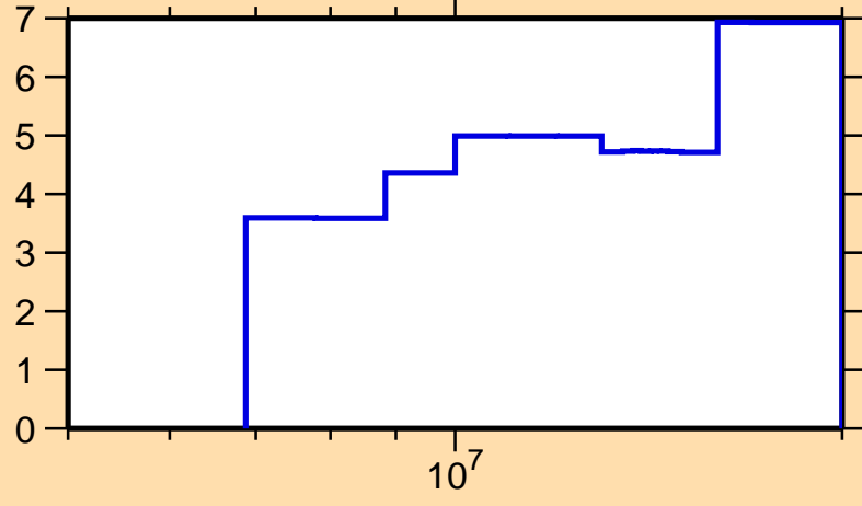
\Delta\sigma/\sigma vs. E for ^{150}\text{Tb}(n,\text{el.})
