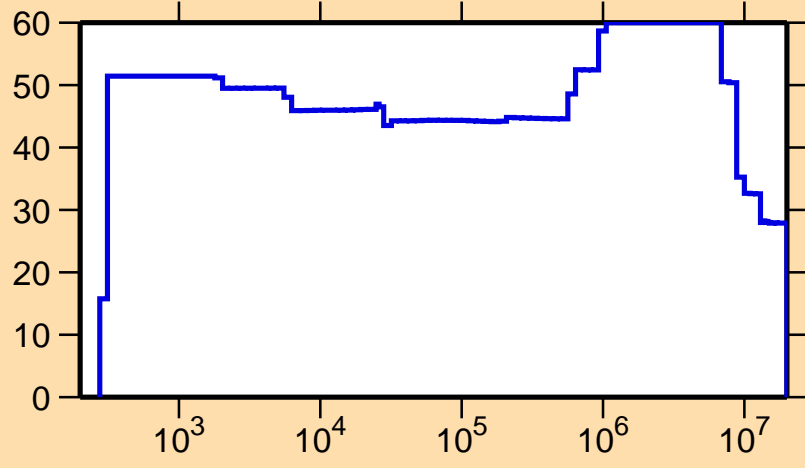
\Delta\sigma/\sigma vs. E for ^{150}\text{Tb}(n,p)
