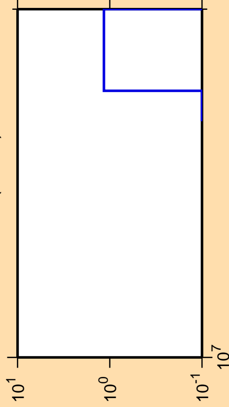
\Delta\sigma/\sigma vs. E for ^{150}\text{Tb} (mt 11)
