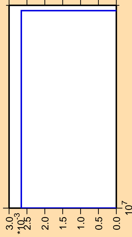
\Delta\sigma/\sigma vs. E for ^{150}\text{Tb}(n,3n\alpha)
