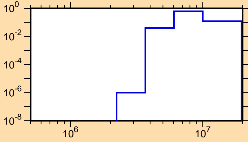
\sigma vs. E for ^{150}\text{Tb}(n,n\alpha)
