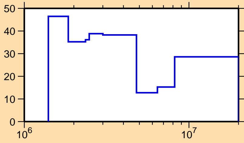
\Delta\sigma/\sigma vs. E for ^{150}\text{Tb}(n,n\text{cont.})
