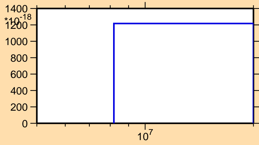
\sigma vs. E for ^{150}\text{Tb}(\text{mt } 11)
