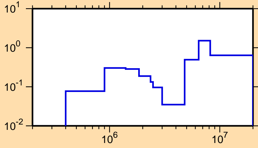
\sigma vs. E for ^{150}\text{Tb}(n,\text{inel.})
