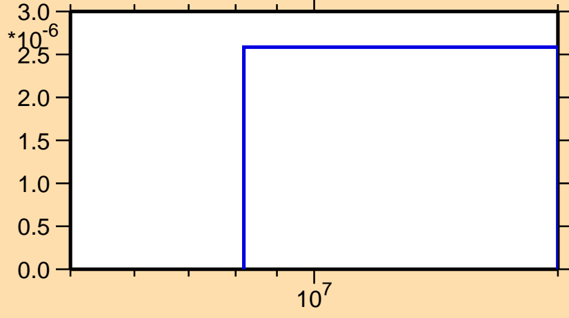
\sigma vs. E for ^{150}\text{Tb}(n,\text{nd})
