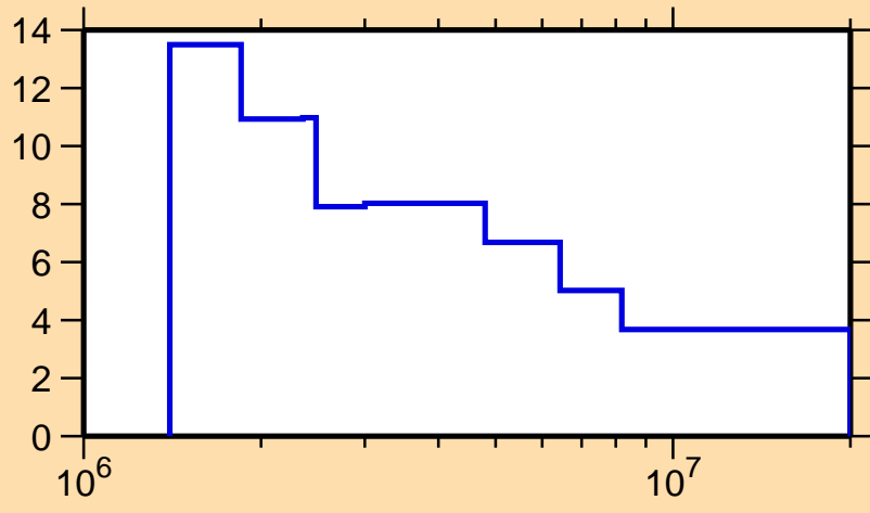
\Delta\sigma/\sigma vs. E for ^{150}\text{Tb}(n,n\text{onel.})
