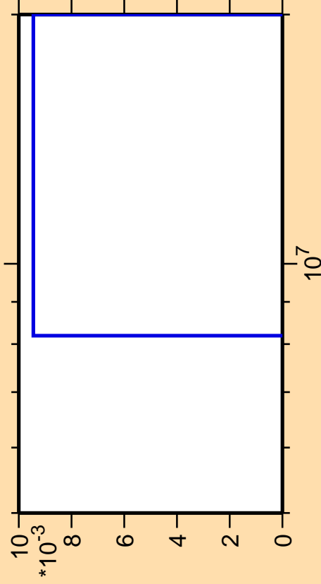
\Delta\sigma/\sigma vs. E for ^{150}\text{Tb}(\text{mt } 11)
