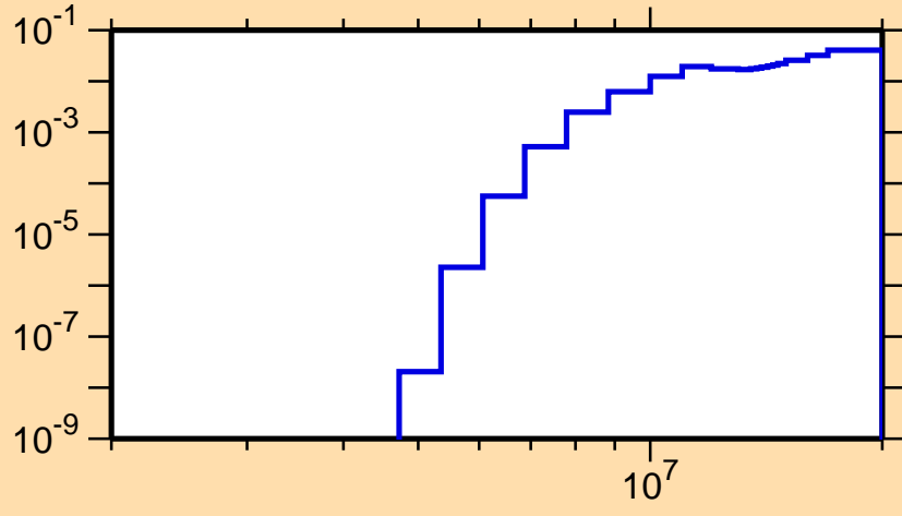
\sigma vs. E for ^{151}\text{Tb}(n,np)
