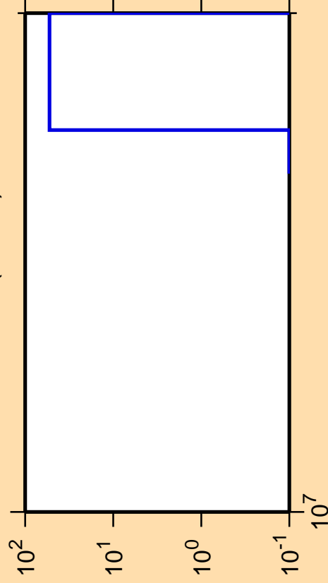
\Delta\sigma/\sigma vs. E for ^{151}\text{Tb} (mt 34)
