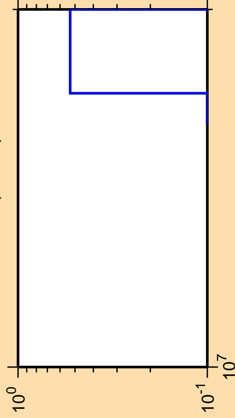
\Delta\sigma/\sigma vs. E for ^{151}\text{Tb} (mt 11)
