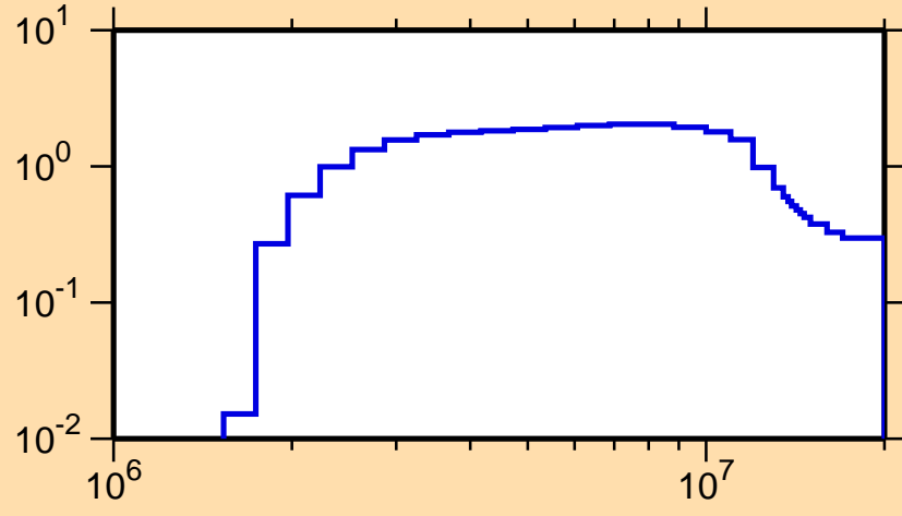
\sigma vs. E for ^{151}\text{Tb}(n,n\text{cont.})
