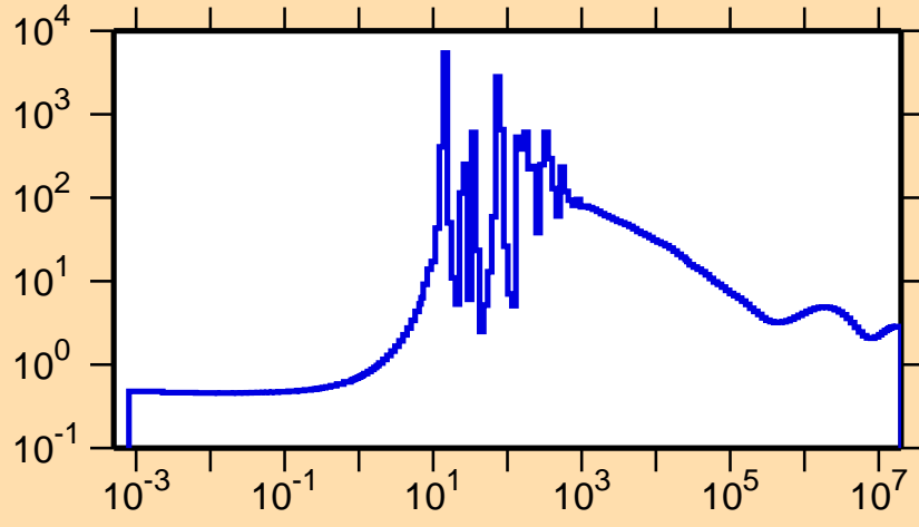
\sigma vs. E for ^{151}\text{Tb}(n,\text{el.})
