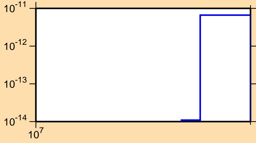
\sigma vs. E for ^{151}\text{Tb} (mt 34)
