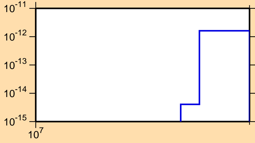
\sigma vs. E for ^{151}\text{Tb}(n,\text{pt})
