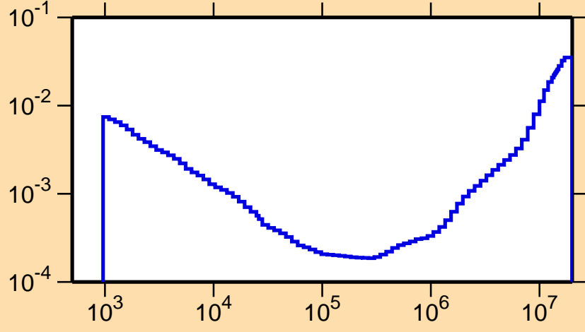
\sigma vs. E for ^{151}\text{Tb}(n,\alpha)
