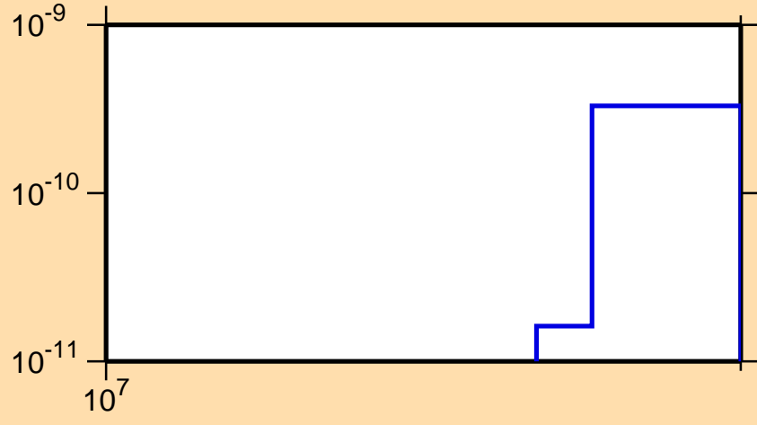
\sigma vs. E for ^{151}\text{Tb}(n,\text{pd})
