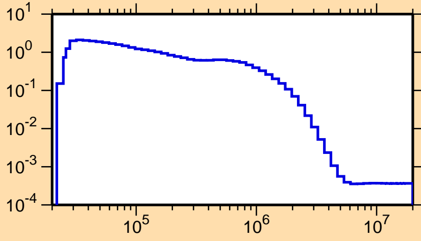
\sigma vs. E for ^{151}\text{Tb}(n,n_1)
