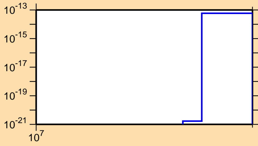
\sigma vs. E for ^{151}\text{Tb} (mt 11)
