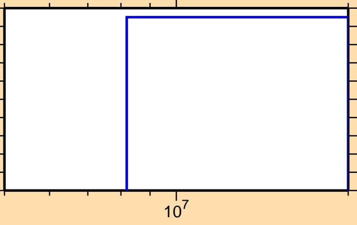
\sigma vs. E for ^{151}\text{Tb}(n,2n\alpha)
