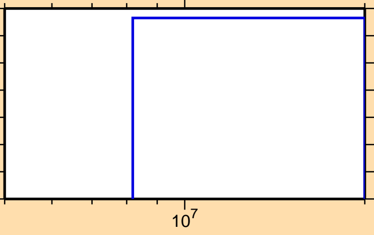
\sigma vs. E for ^{151}\text{Tb}(n,\text{pt})
