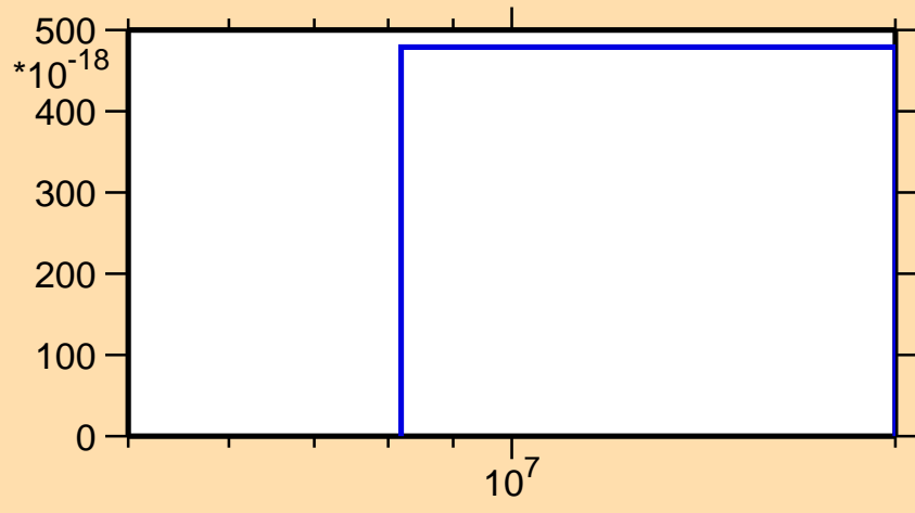
\sigma vs. E for ^{151}\text{Tb}(\text{mt } 11)
