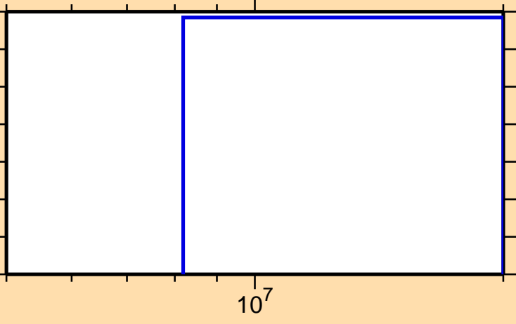
\sigma vs. E for ^{151}\text{Tb}(n,2np)
