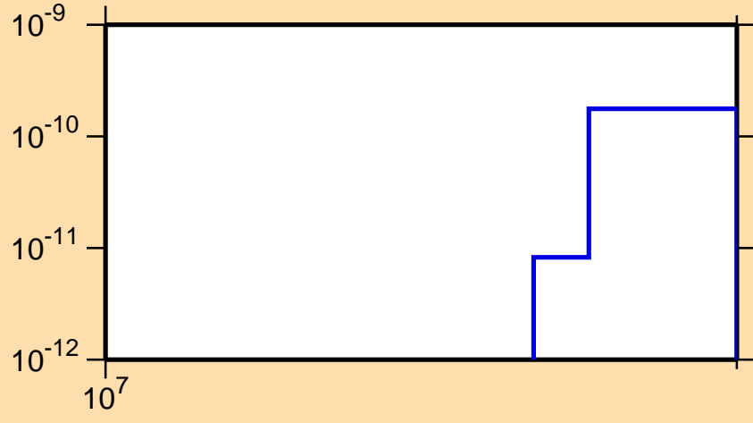
\sigma vs. E for ^{151}\text{Tb}(n,pd)
