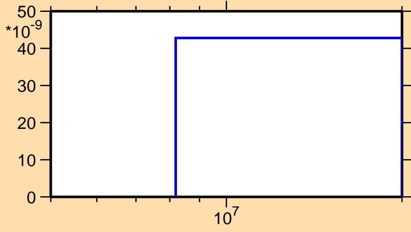
\sigma vs. E for ^{151}\text{Tb} (mt 45)
