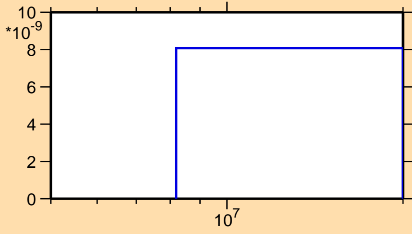
\sigma vs. E for ^{151}\text{Tb}(\text{mt117})
