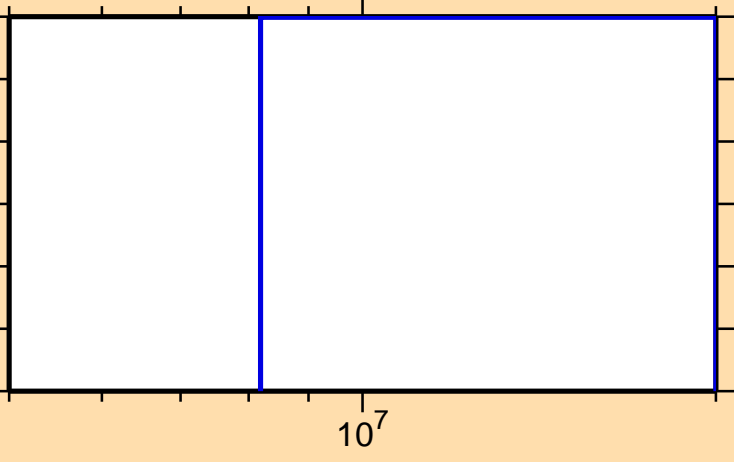
\sigma vs. E for ^{151}\text{Tb}(n,nt)
