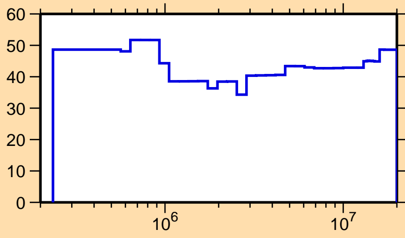
\Delta\sigma/\sigma vs. E for ^{152}\text{Tb}(n,n_1)
