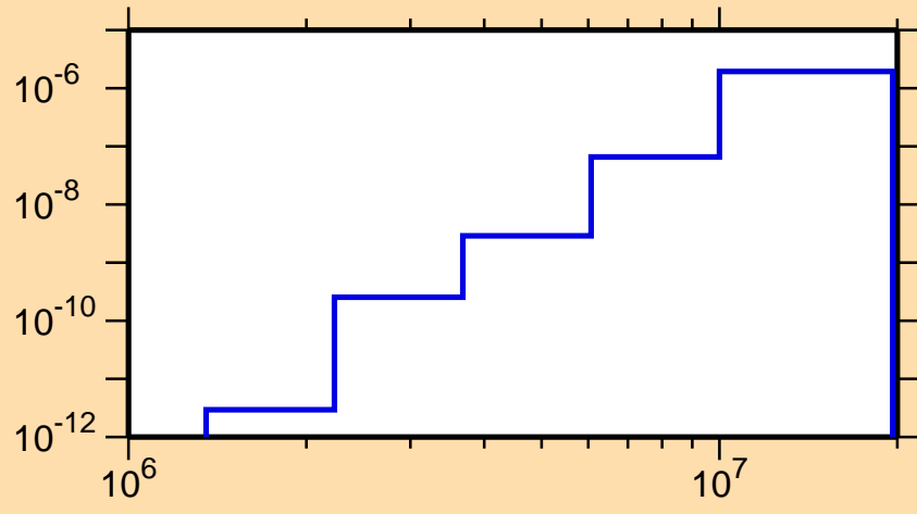
\sigma vs. E for ^{152}\text{Tb}(n,p\alpha)
