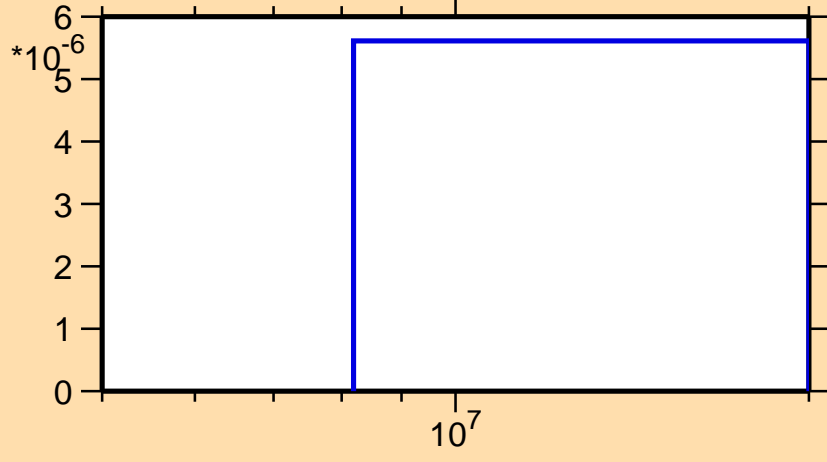
\sigma vs. E for ^{152}\text{Tb}(n,\text{nd})
