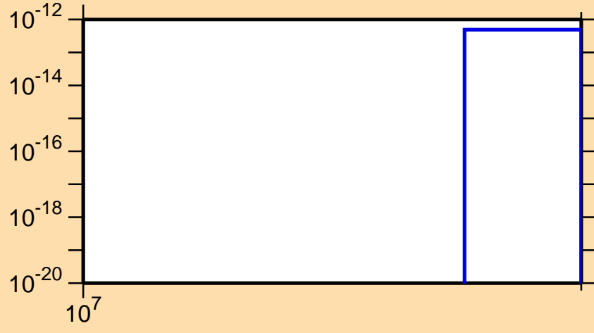
\sigma vs. E for ^{152}\text{Tb} (mt 11)
