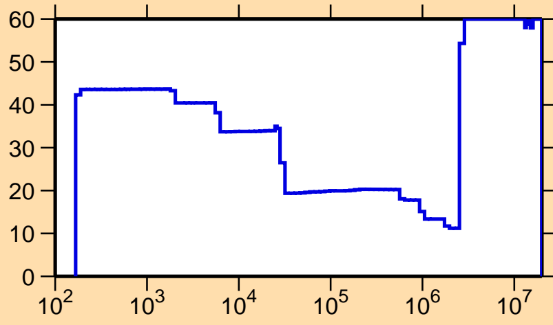
\Delta\sigma/\sigma vs. E for ^{152}\text{Tb}(n,\gamma)
