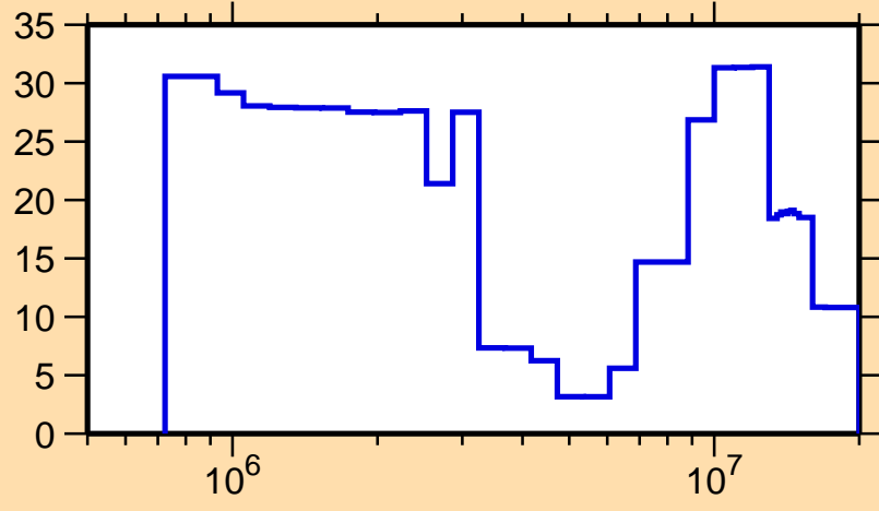
\Delta\sigma/\sigma vs. E for ^{152}\text{Tb}(n,n\text{cont.})
