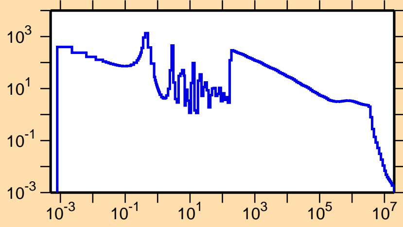
\sigma vs. E for ^{152}\text{Tb}(n,\gamma)
