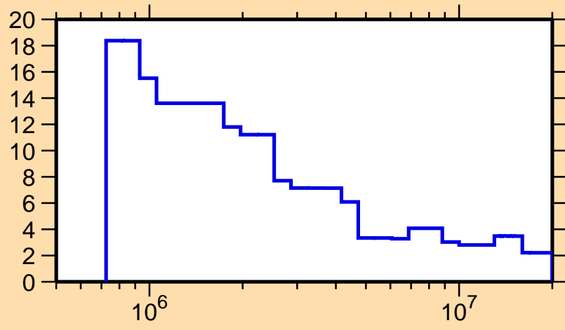
\Delta\sigma/\sigma vs. E for ^{152}\text{Tb}(n,n\text{onel.})
