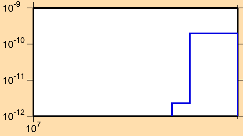
\sigma vs. E for ^{152}\text{Tb} (mt 34)
