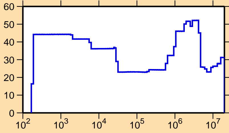
\Delta\sigma/\sigma vs. E for ^{152}\text{Tb}(n,p)
