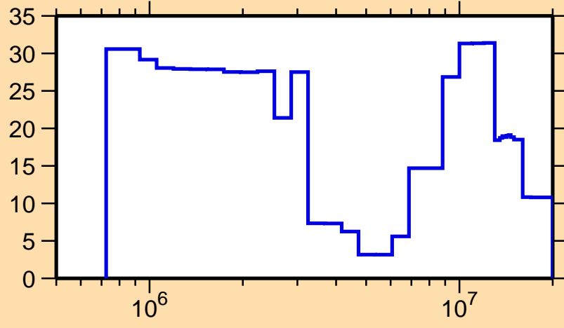
\Delta\sigma/\sigma vs. E for ^{152}\text{Tb}(n,n\text{cont.})
