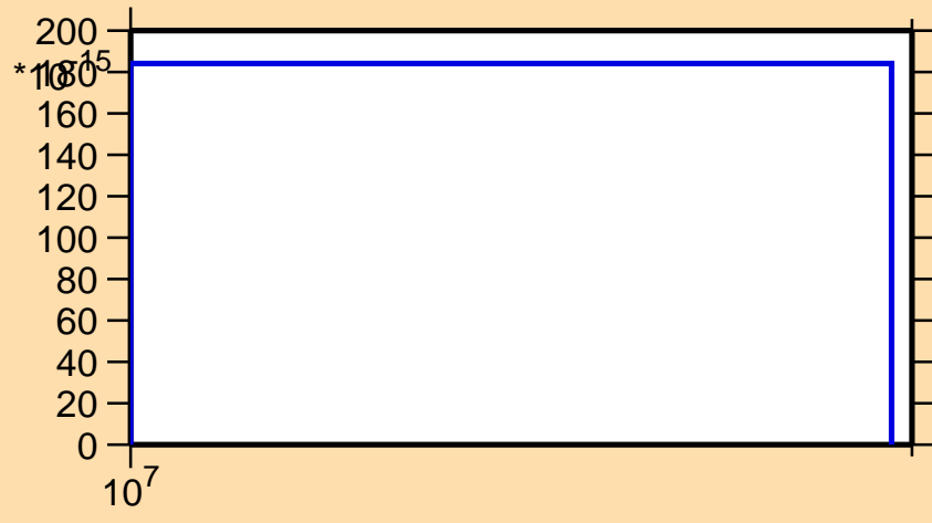
\sigma vs. E for ^{152}\text{Tb}(n,pd)
