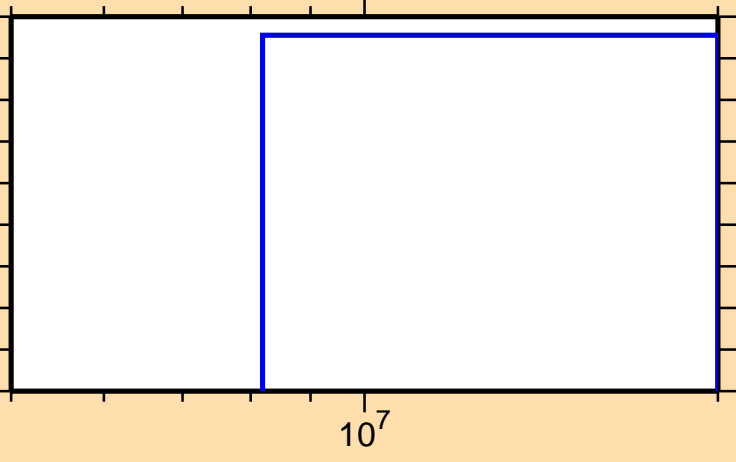
\sigma vs. E for ^{152}\text{Tb} (mt 34)
