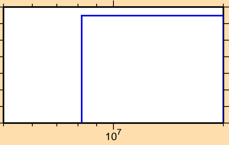
\sigma vs. E for ^{152}\text{Tb}(\text{mt117})
