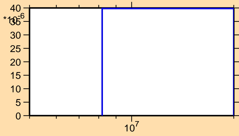
\sigma vs. E for ^{152}\text{Tb}(n,2np)
