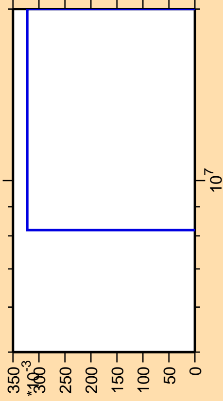
\Delta\sigma/\sigma vs. E for ^{152}\text{Tb}(n,pd)
