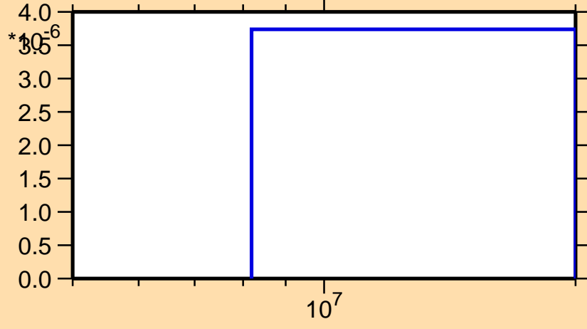
\sigma vs. E for ^{152}\text{Tb}(n,\text{nd})
