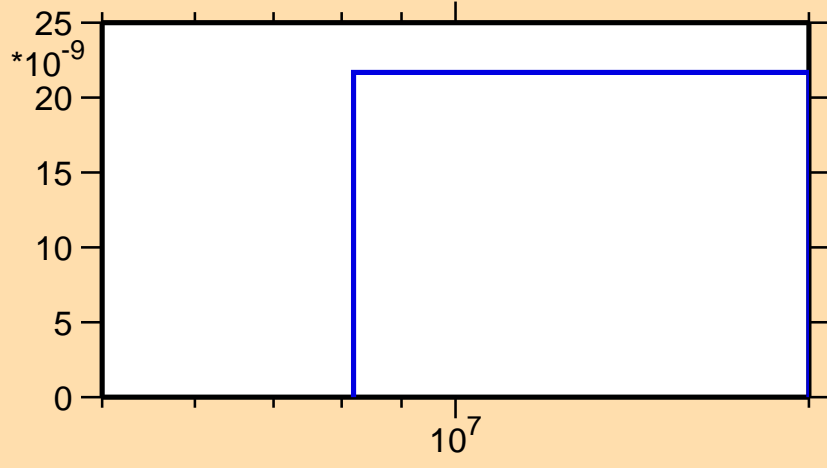
\sigma vs. E for ^{152}\text{Tb} (mt 45)
