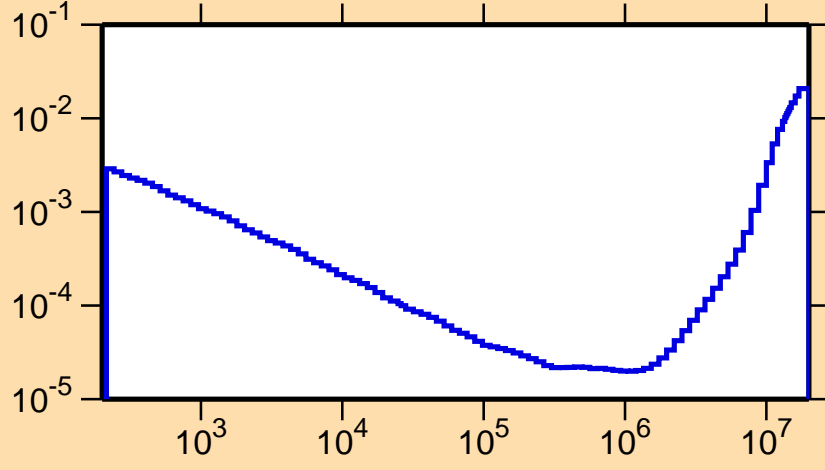
\sigma vs. E for ^{153}\text{Tb}(n,\alpha)
