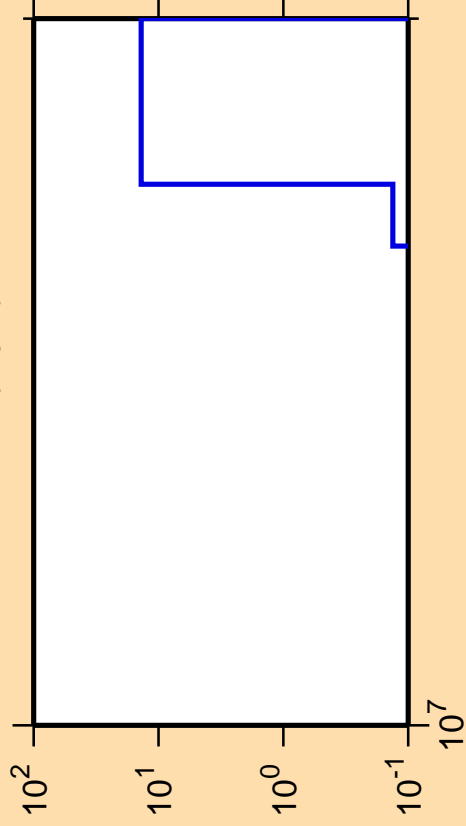
\Delta\sigma/\sigma vs. E for ^{153}\text{Tb}(n,pd)
