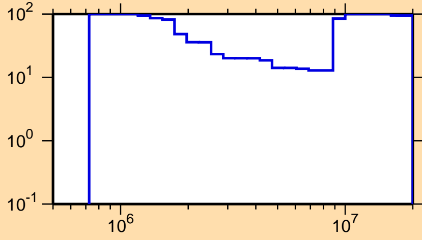
\Delta\sigma/\sigma vs. E for ^{153}\text{Tb}(n,n\text{cont.})
