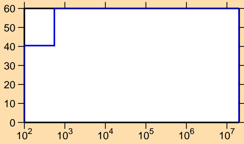
\Delta\sigma/\sigma vs. E for ^{153}\text{Tb}(n,p)
