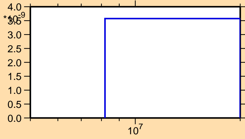
\sigma vs. E for ^{153}\text{Tb} (mt 45)
