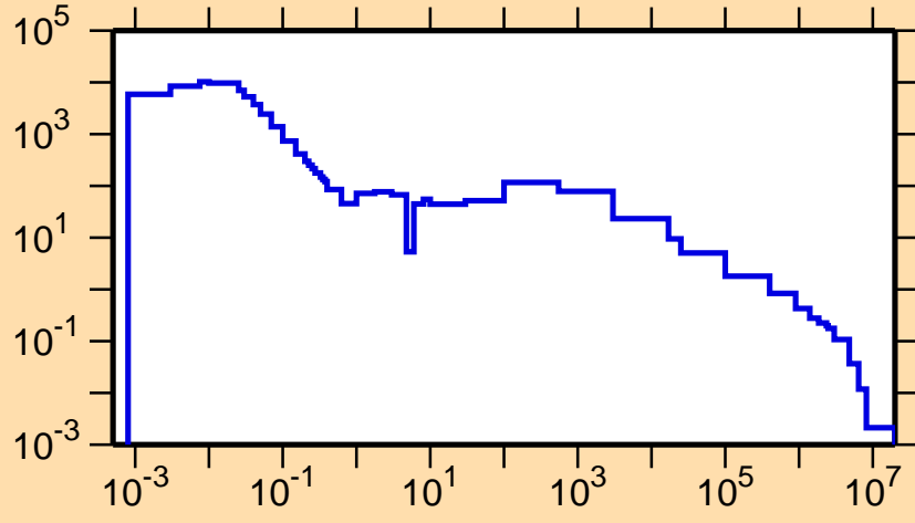
\sigma vs. E for ^{153}\text{Tb}(n,\gamma)
