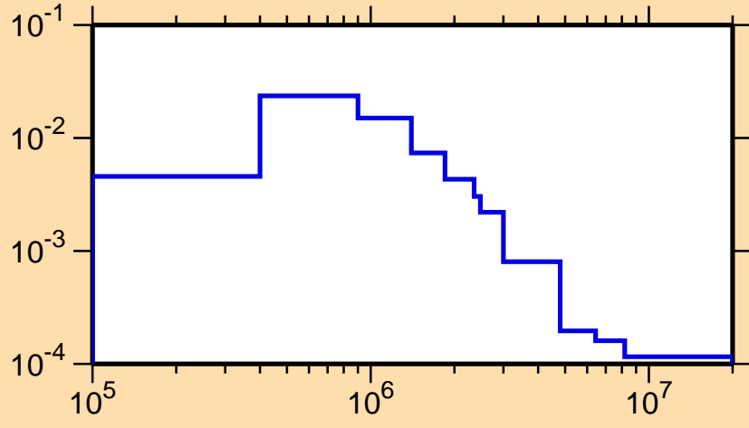
\sigma vs. E for ^{153}\text{Tb}(n,n_3)
