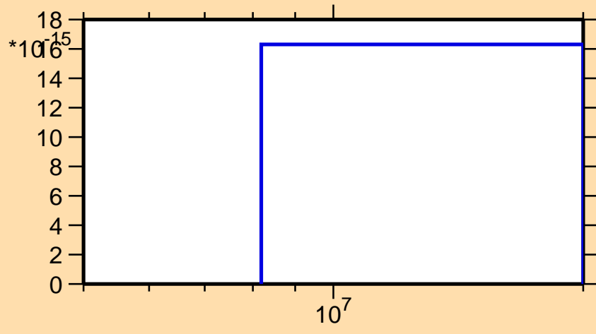
\sigma vs. E for ^{153}\text{Tb}(n,pd)
