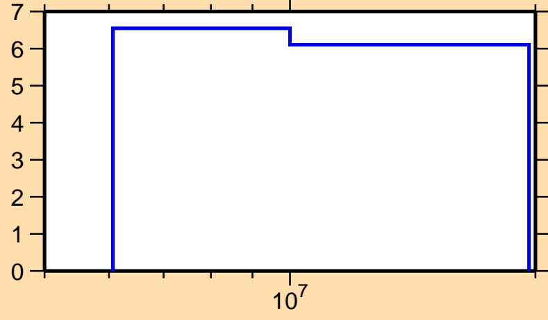
\Delta\sigma/\sigma vs. E for ^{154}\text{Tb}(n,\text{nonel.})
