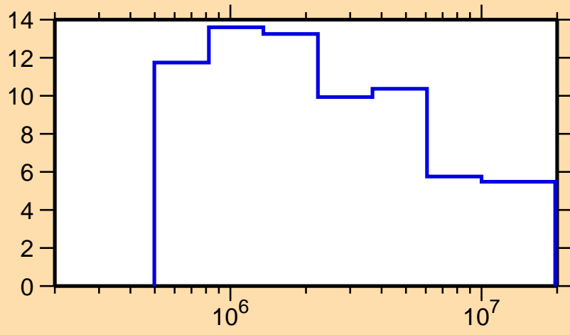
\Delta\sigma/\sigma vs. E for ^{154}\text{Tb}(n,\text{tot.})
