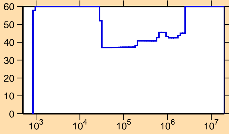
\Delta\sigma/\sigma vs. E for ^{154}\text{Tb}(n,\gamma)
