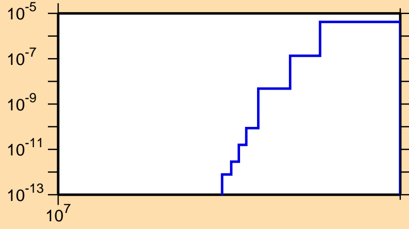
\sigma vs. E for ^{154}\text{Tb}(n,nt)
