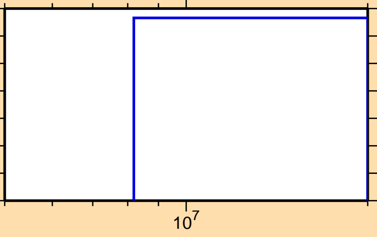
\sigma vs. E for ^{154}\text{Tb}(n,2n\alpha)
