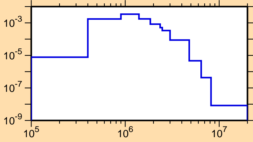
\sigma vs. E for ^{154}\text{Tb}(n,n_2)
