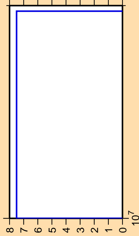
\Delta\sigma/\sigma vs. E for ^{154}\text{Tb}(n,3n\alpha)
