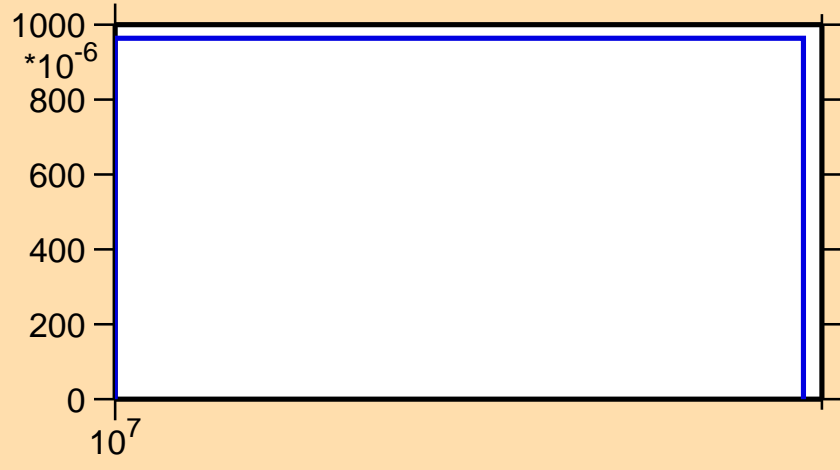
\sigma vs. E for ^{154}\text{Tb}(n,3n)
