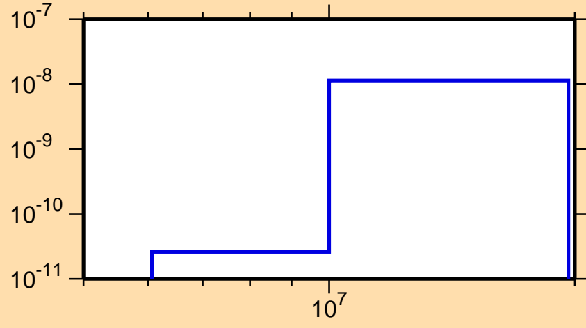
\sigma vs. E for ^{154}\text{Tb}(n,p\alpha)
