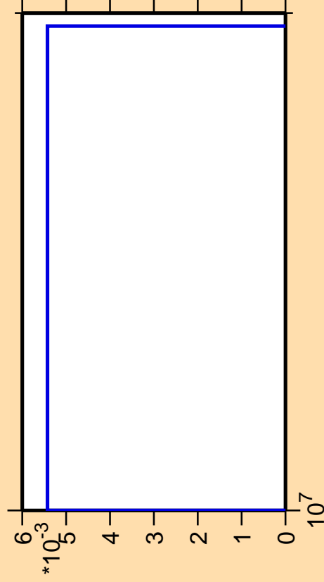
\Delta\sigma/\sigma vs. E for ^{154}\text{Tb} (mt 11)
