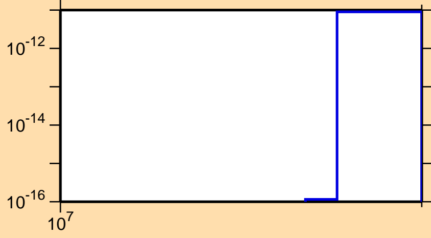
\sigma vs. E for ^{155}\text{Tb}(n,3n\alpha)
