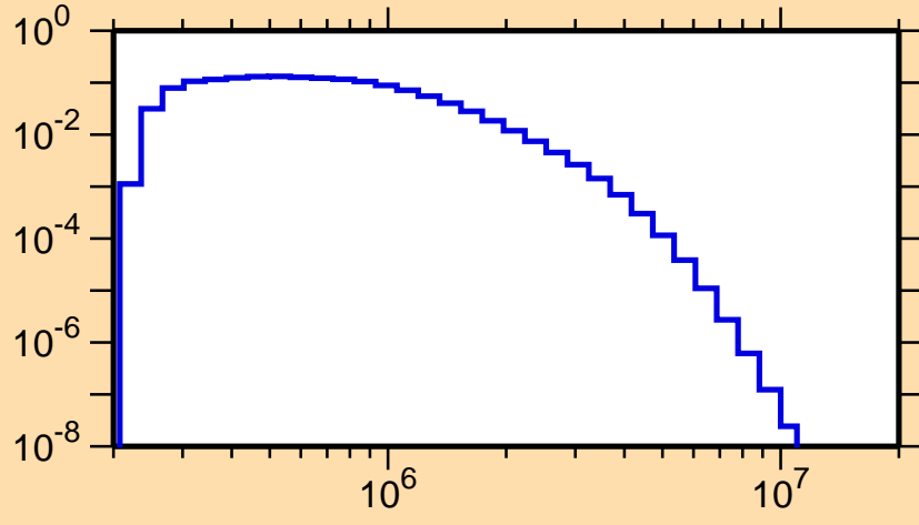
\sigma vs. E for ^{155}\text{Tb}(n,n_3)
