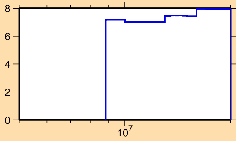
\Delta\sigma/\sigma vs. E for ^{155}\text{Tb}(n,\text{nonel.})
