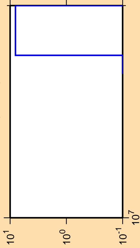
\Delta\sigma/\sigma vs. E for ^{155}\text{Tb}(n,3n\alpha)
