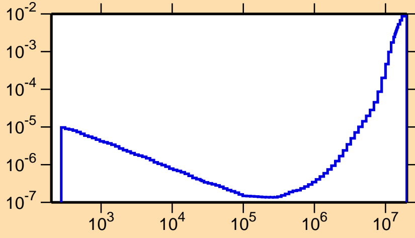
\sigma vs. E for ^{155}\text{Tb}(n,\alpha)
