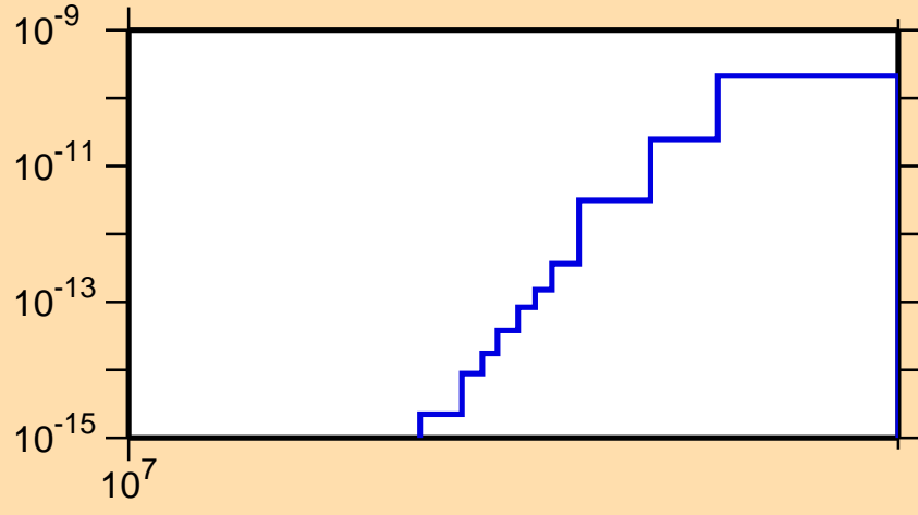
\sigma vs. E for ^{155}\text{Tb} (mt 45)
