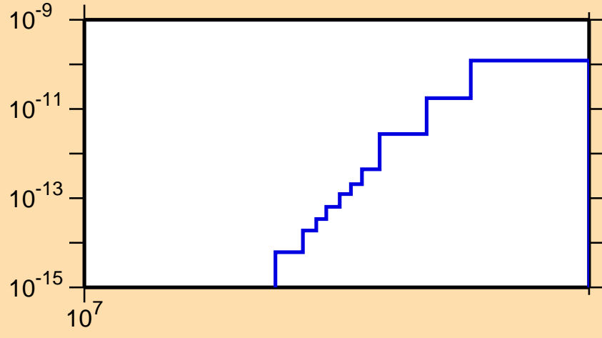
\sigma vs. E for ^{155}\text{Tb}(\text{mt117})
