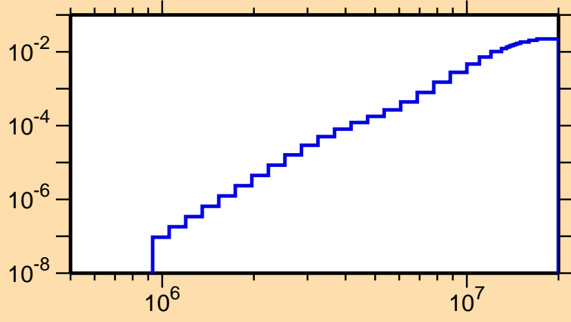
\sigma vs. E for ^{155}\text{Tb}(n,p)
