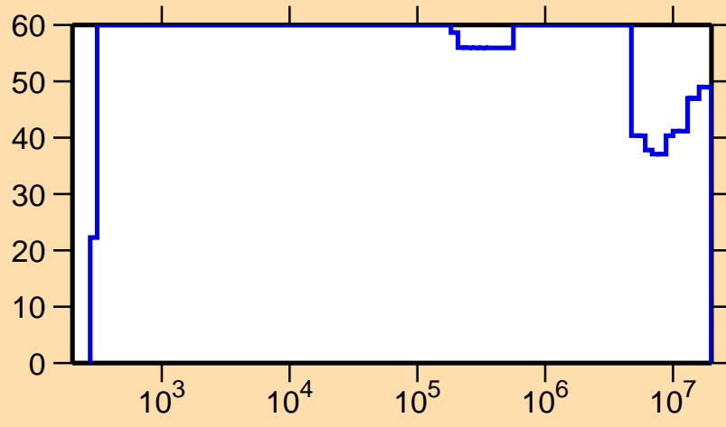
\Delta\sigma/\sigma vs. E for ^{155}\text{Tb}(n,p)
