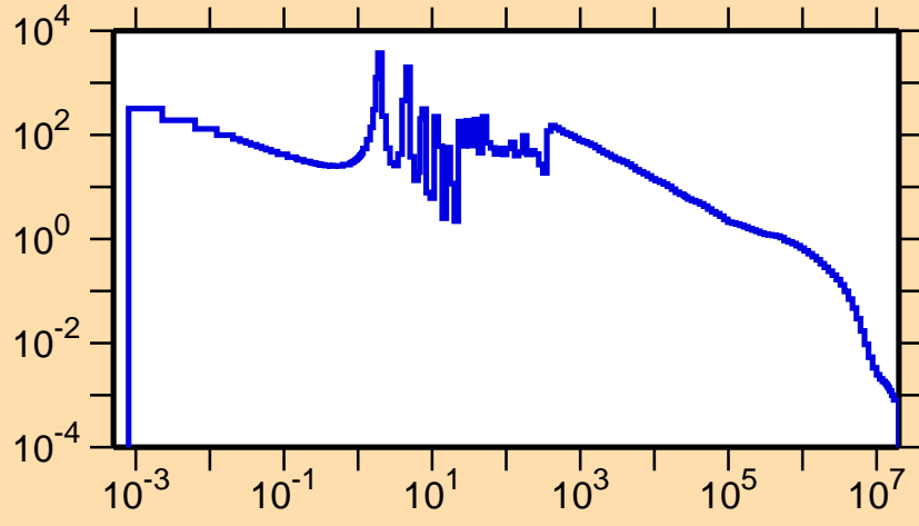
\sigma vs. E for ^{155}\text{Tb}(n,\gamma)
