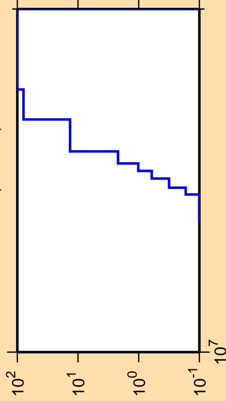
\Delta\sigma/\sigma vs. E for ^{155}\text{Tb}(\text{mt117})
