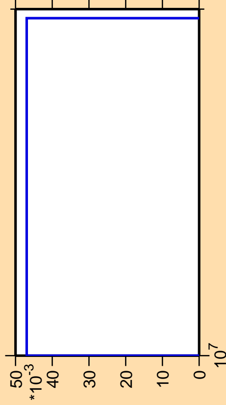
\Delta\sigma/\sigma vs. E for ^{155}\text{Tb}(n,3n\alpha)
