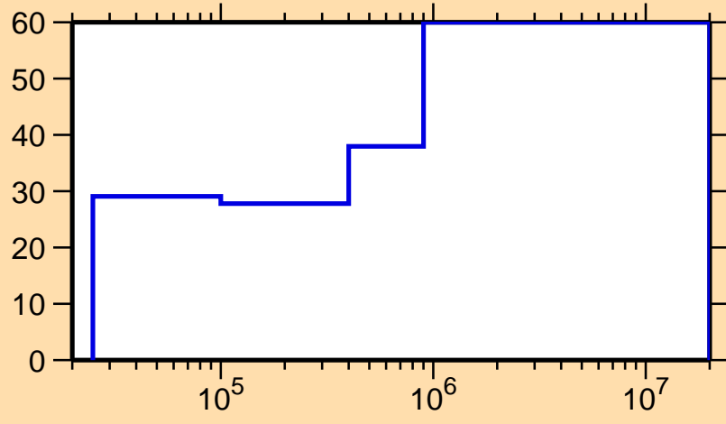
\Delta\sigma/\sigma vs. E for ^{155}\text{Tb}(n,n_1)
