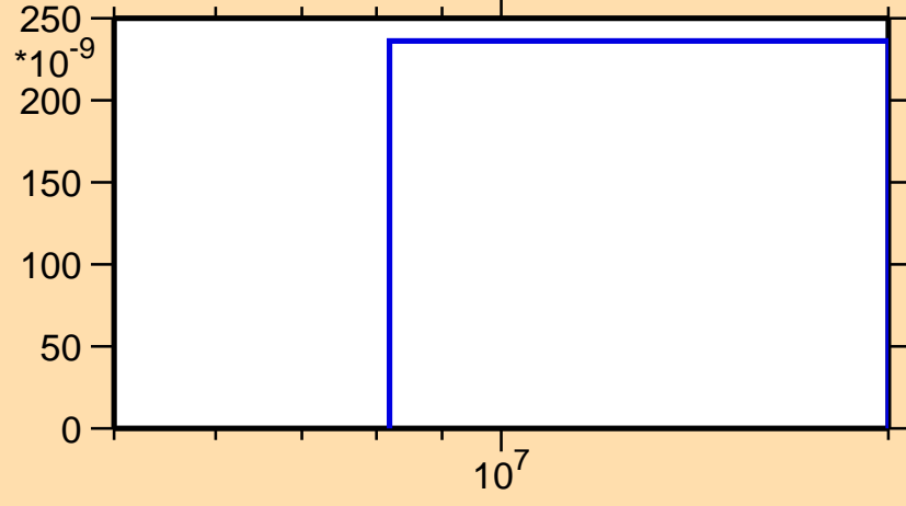
\sigma vs. E for ^{155}\text{Tb}(n,2n\alpha)
