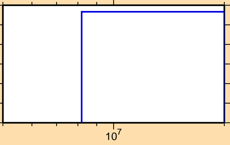
\sigma vs. E for ^{155}\text{Tb}(n,nt)
