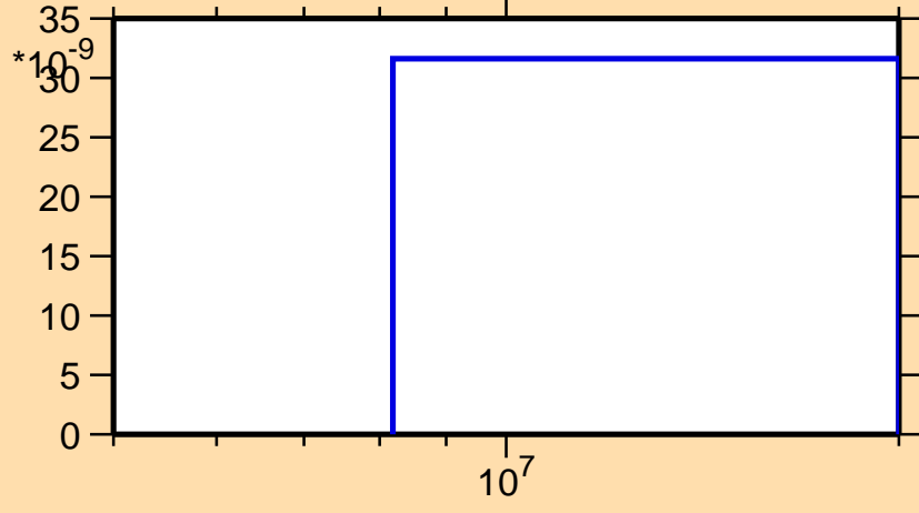
\sigma vs. E for ^{155}\text{Tb}(n,\text{nd})
