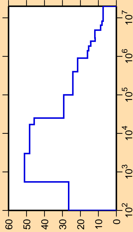
\Delta\sigma/\sigma vs. E for ^{155}\text{Tb}(n,\text{nonel.})
