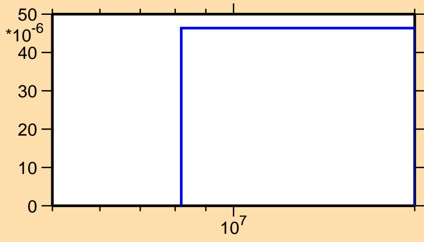
\sigma vs. E for ^{155}\text{Tb}(n,t)
