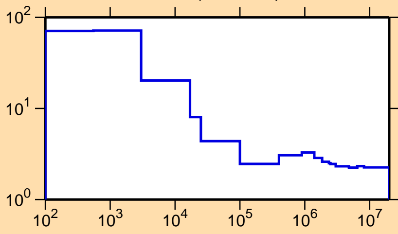
\sigma vs. E for ^{155}\text{Tb}(n,\text{nonel.})
