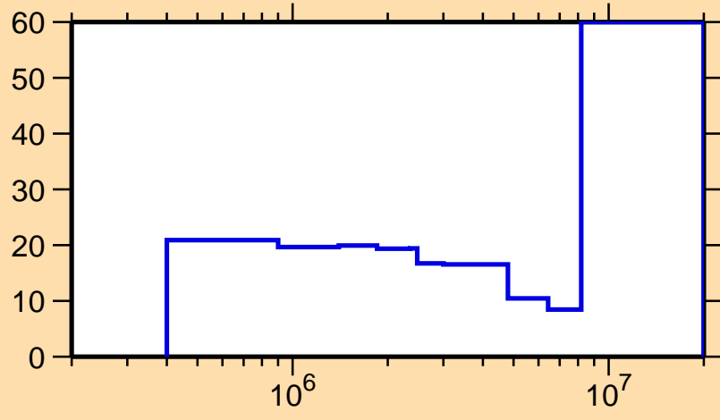
\Delta\sigma/\sigma vs. E for ^{155}\text{Tb}(n,\text{inel.})
